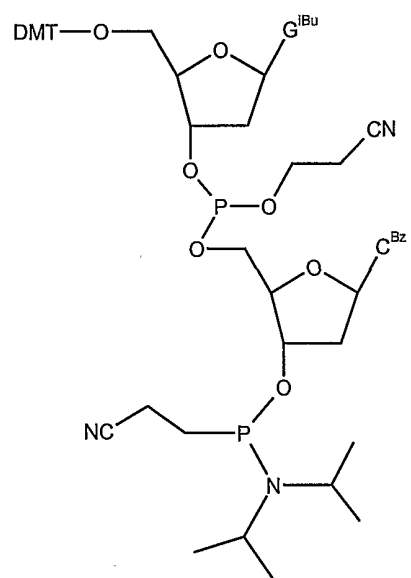
Trivalent phosphorous dimer
