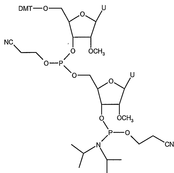
Figure 3: 2'-O-Methyl Dimer prepared in Example 2.
