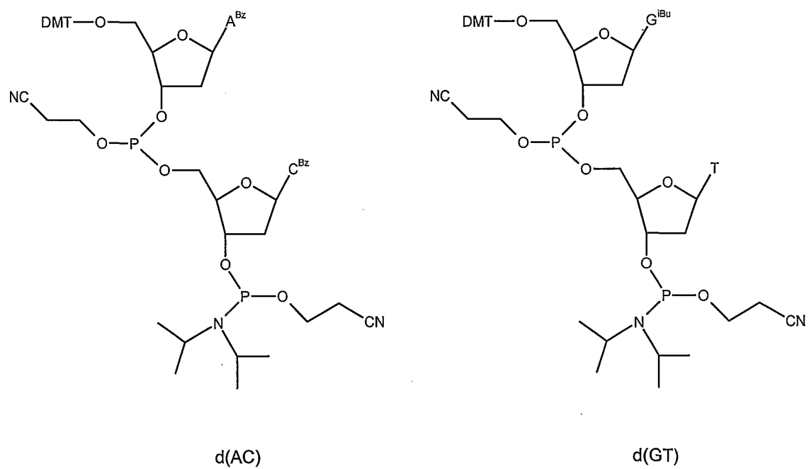
Figure 4: Dimers used to synthesize oligonucleotides in Example 4.
