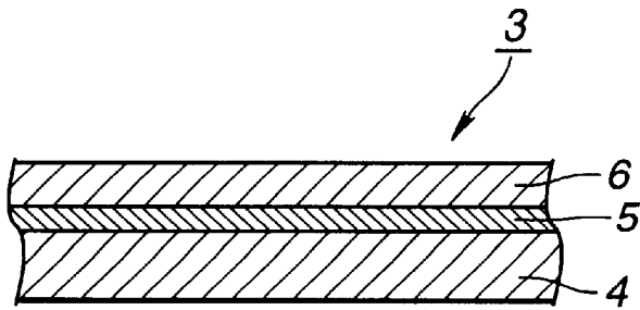
CROSS SECTIONAL VIEW SHOWING ESSENTIAL PORTION OF HOLOGRAM RECORDING MEDIUM
