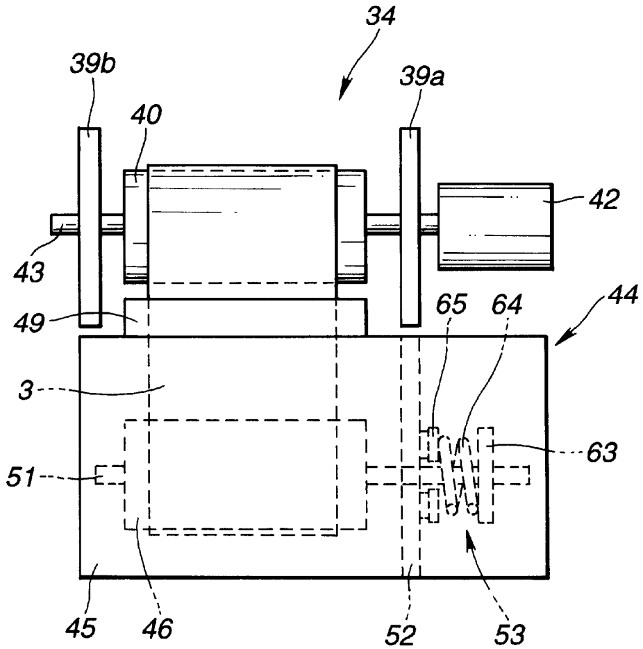
FRONT VIEW SHOWING CARTRIDGE FOR HOLOGRAM-IMAGE RECORDING MEDIUM AND RECORDING-MEDIUM FEEDING MECHANISM
