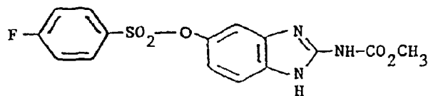
Luxobendazole
