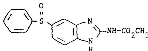
Oxfendazole
