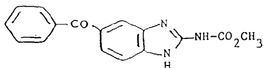
Mebendazole
