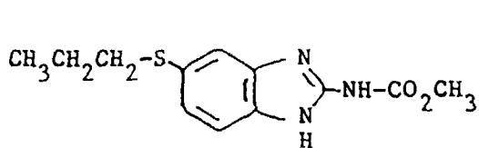
Albendazole
