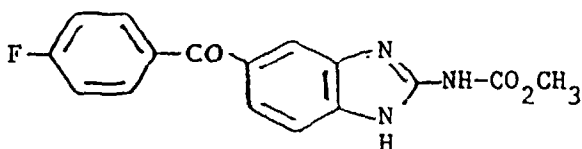
Flubendazole
