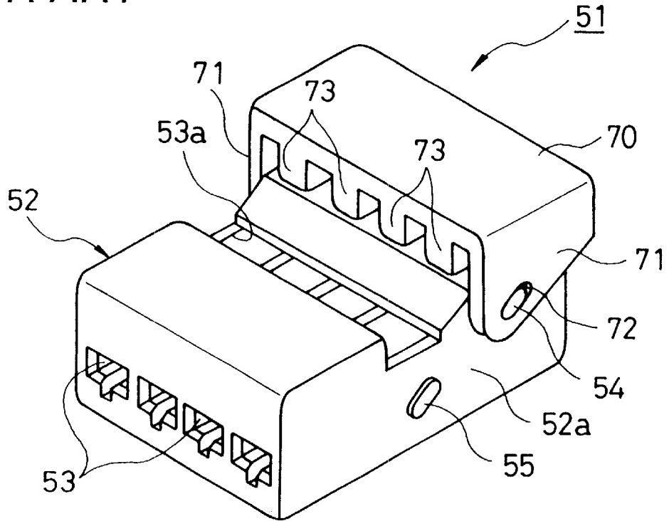
FIG. 11 PRIOR ART
