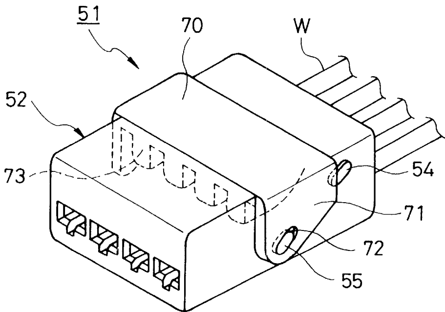
FIG. 11 PRIOR ART
