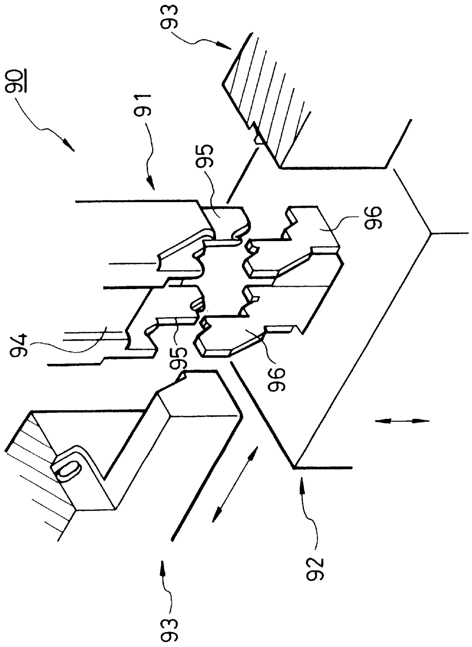
FIG. 14 PRIOR ART
