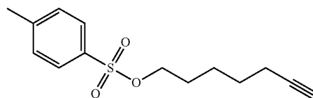
Hep-6-yn-1-yl 4-methylbenzenesulfonate
