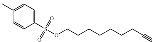
Non-8-yn-1-yl 4-methylbenzenesulfonate
