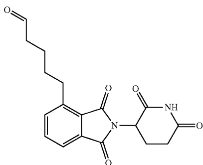
5-(2-(2,6-Dioxopiperidin-3-yl)-1,3-dioxoisindolin-4-yl)pentanal
