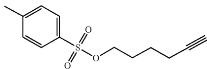
Hex-5-yn-1-yl 4-methylbenzenesulfonate
