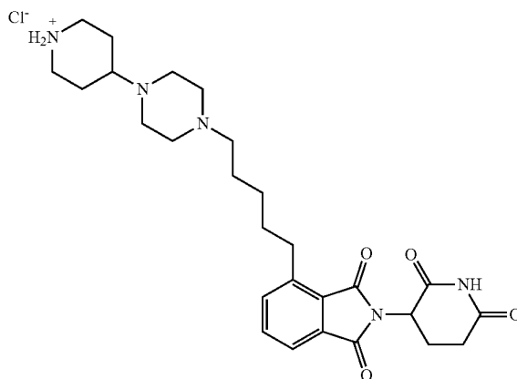
4-(4-(5-(2-(2,6-Dioxopiperidin-3-yl)-1,3-dioxoisindolin-4-yl)pentyl)piperazin-1-yl)piperidine-1-ium hydrochloride
