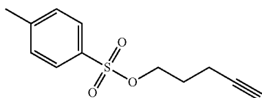
Pent-4-yn-1-yl 4-methylbenzenesulfonate
