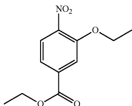
Ethyl 3-ethoxy-4-nitrobenzoate
