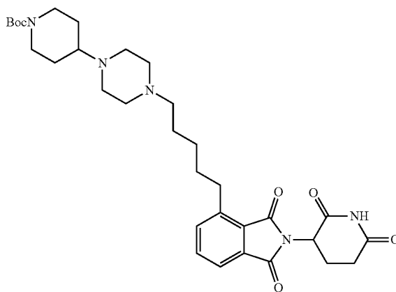
tert-Butyl 4-(4-(5-(2-(2,6-dioxopiperidin-3-yl)-1,3-dioxoisindolin-4-yl)pentyl)piperazin-1-yl)piperidine-1-carboxylate
