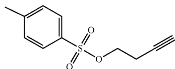
But-3-yn-1-yl 4-methylbenzenesulfonate
