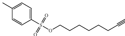
Oct-7-yn-1-yl 4-methylbenzenesulfonate
