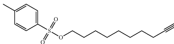
Dec-9-yn-1-yl 4-methylbenzenesulfonate
