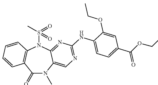
Ethyl 3-ethoxy-4-((5-methyl-11-(methylsulfonyl)-6-oxo-6,11-dihydro-5H-benzo[e]pyrimido[5,4-b][1,4]diazepin-2-yl)amino)benzoate
