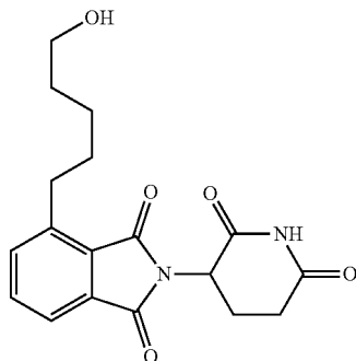
2-(2,6-Dioxopiperidin-3-yl)-4-(5-hydroxypentyl)isoindoline-1,3-dione
