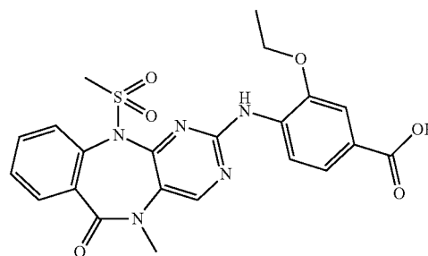
3-Ethoxy-4-((5-methyl-11-(methylsulfonyl)-6-oxo-6,11-dihydro-5H-benzo[e]pyrimido[5,4-b][1,4]diazepin-2-yl)amino)benzoic acid
