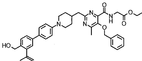
[Chemical 149]
