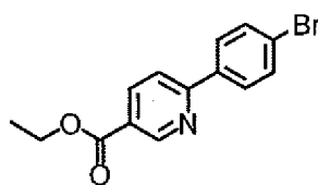
[Chemical 63]
