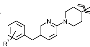
(1B-7)
