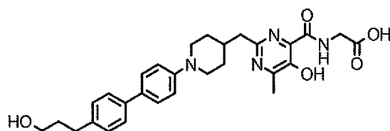
[Chemical 144]
