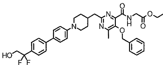
[Chemical 106]
