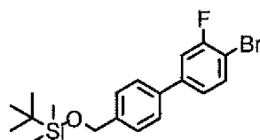
[Chemical 126]
