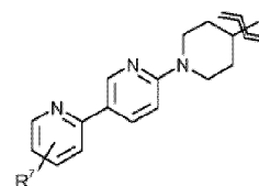
(1B-4)
