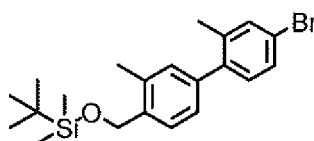
[Chemical 98]
