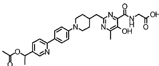
[Chemical 57]
