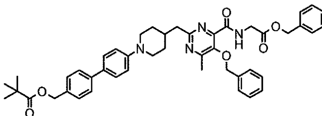
[Chemical 116]
