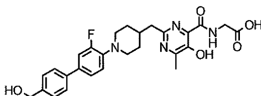
[Chemical 125]
