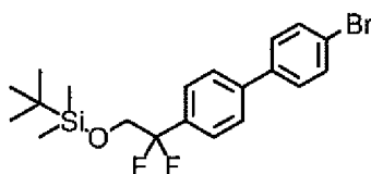
[Chemical 105]
