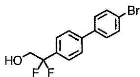
[Chemical 104]
