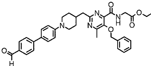
[Chemical 132]
