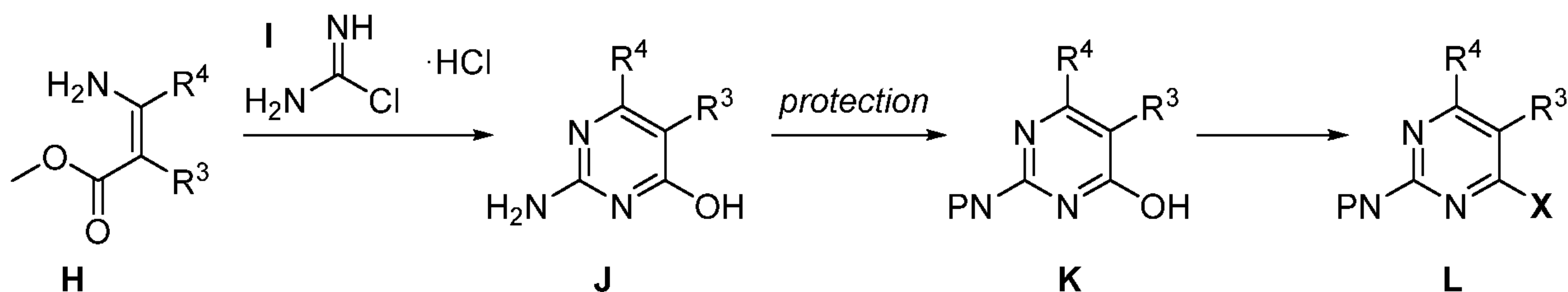
Scheme 3. Preparation of electrophile B , e.g., an N -protected B , i.e. L
