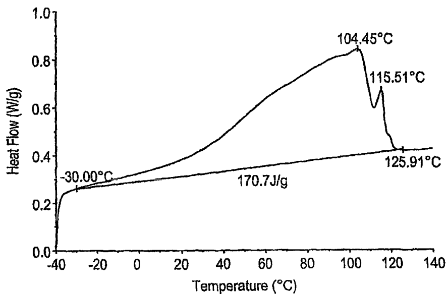
FIG. 6 DSC Example 4
