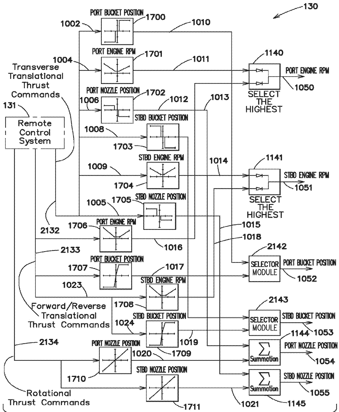
TWIN WATERJET SIGNAL DIAGRAM REMOTELY CONTROLLED
