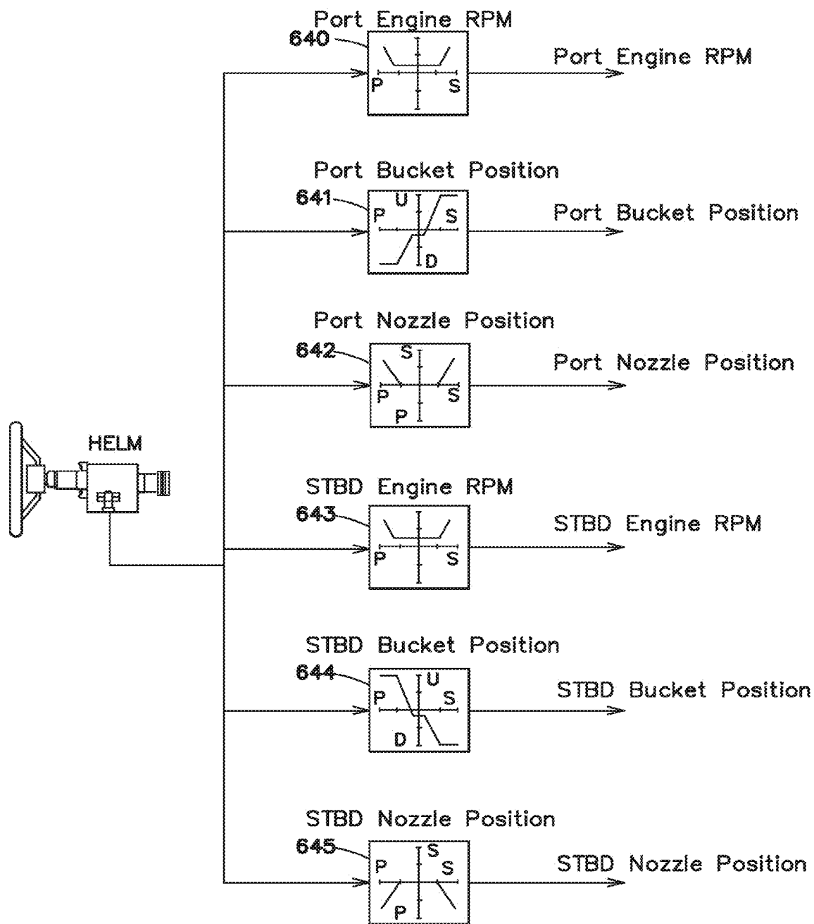
Integrated Twin Waterjet Signal Diagram: Zone 3 (Rotation Only (Joystick Centered))
