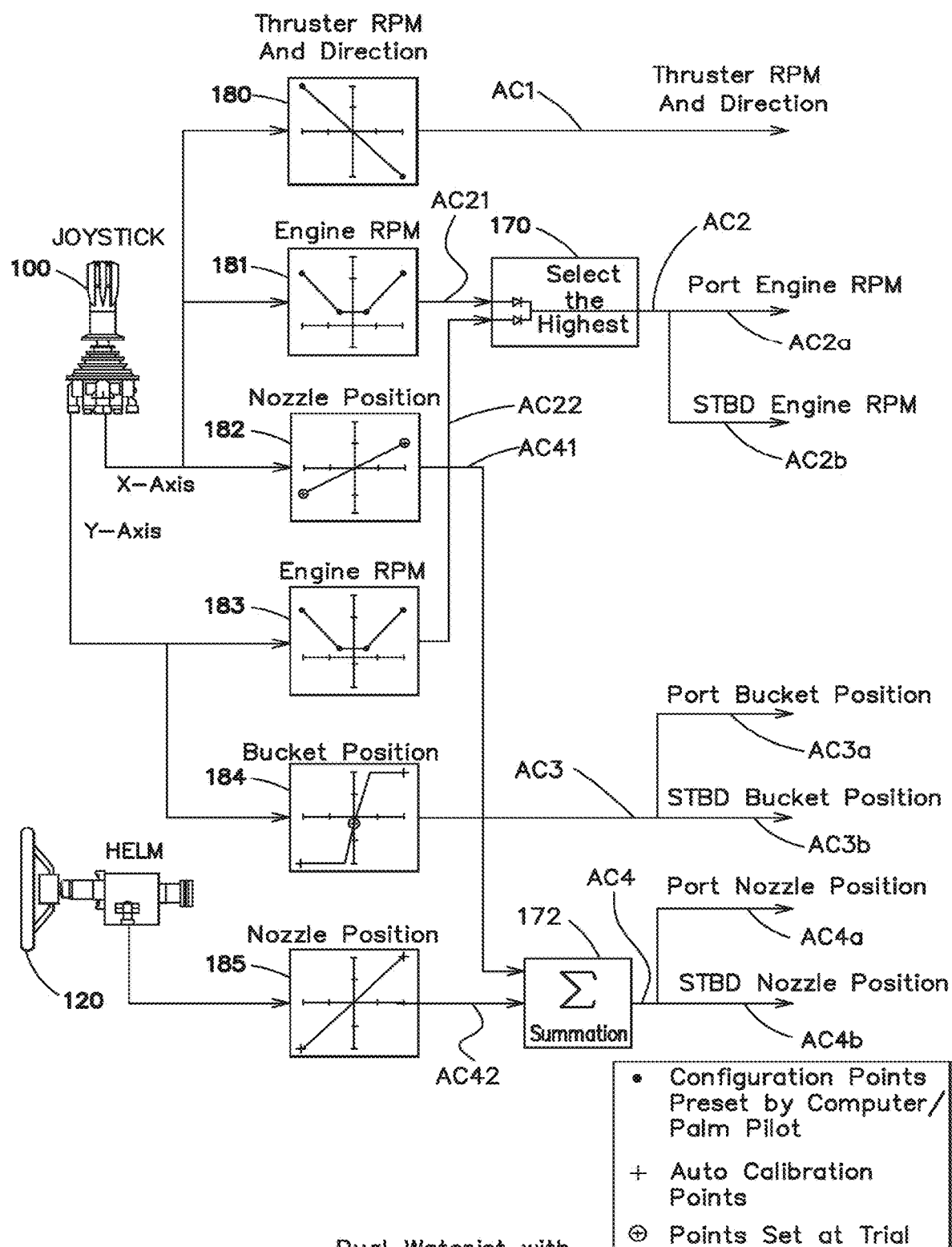
Dual Waterjet with Bow Thruster Signal Diagram
