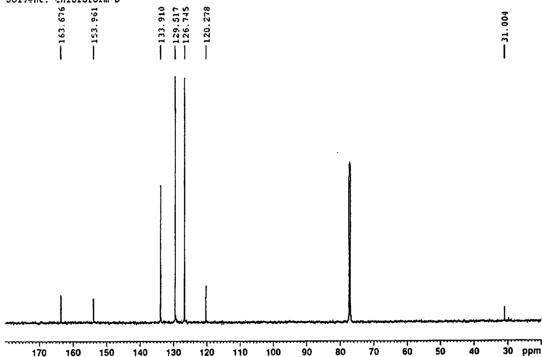
FIG. 8 13 C NMR spectrum of PDO.
