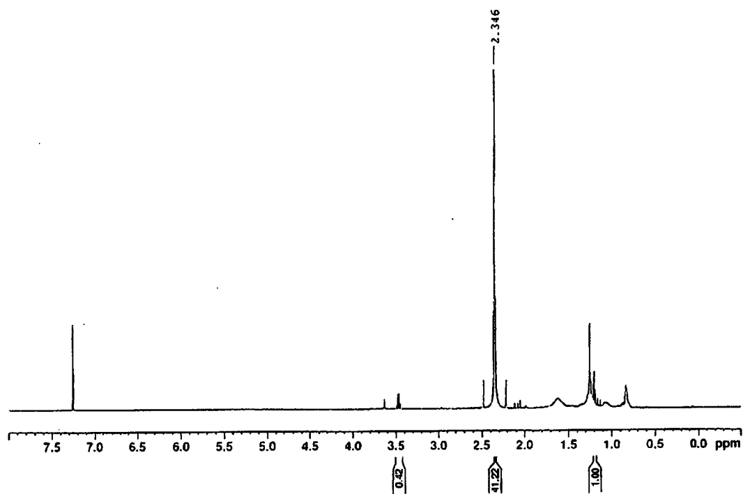
FIG. 4 ^1\text{H} NMR SPECTRUM of MDO.
