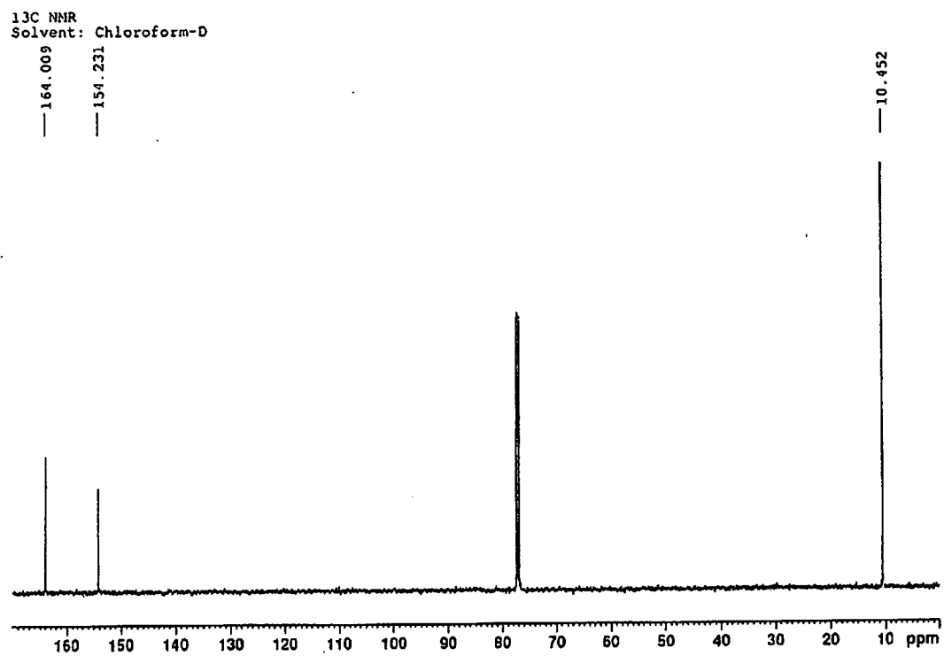
FIG 5. 13 C NMR spectrum of MDO.
