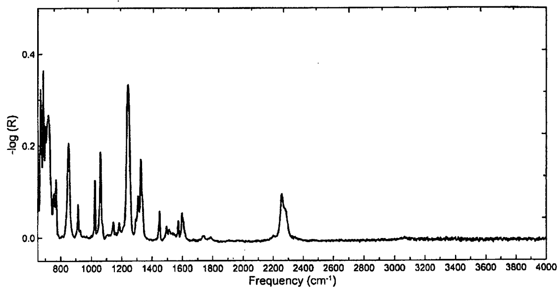
FIG. 12 FTIR spectrum of BS.
