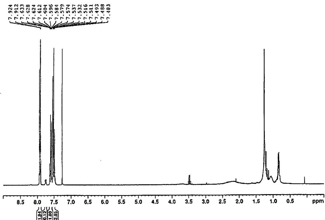
FIG. 10 1 H NMR spectrum of BS.
