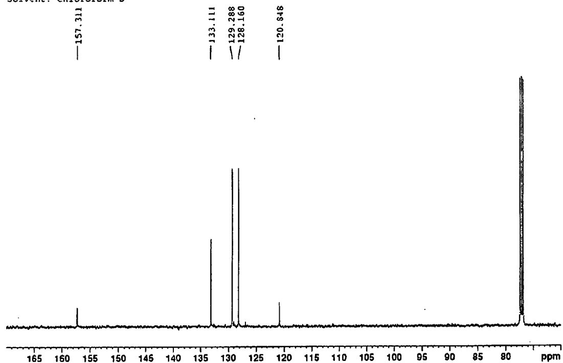
FIG. 11 ^{13}\text{C} NMR spectrum of BS.
