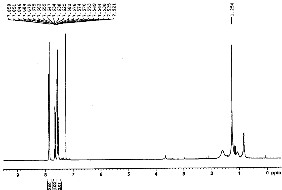
FIG. 7 1 H NMR spectrum of PDO.
