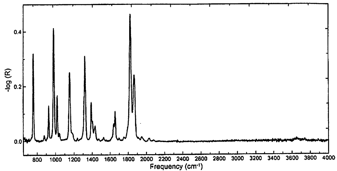
FIG 6. FTIR spectrum of MDO.
