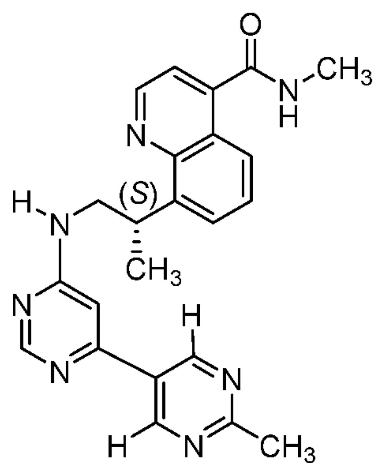
(Compound 1),
