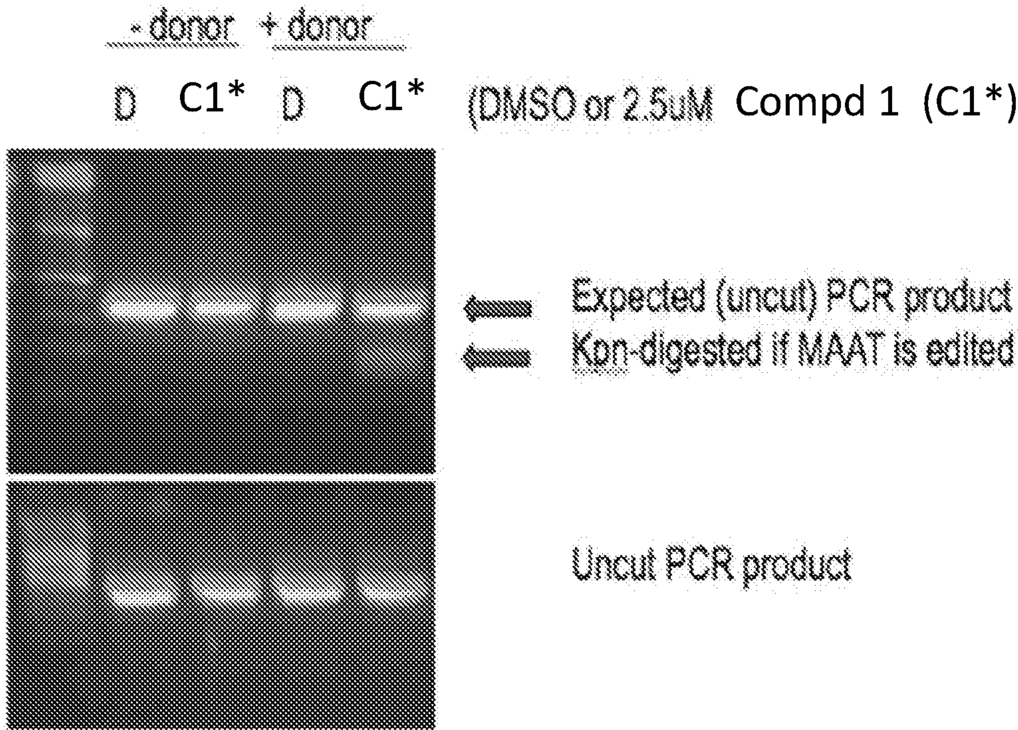
Z3 MAAT guide +/- asymmetric donor with introduced KpnI site Huh7 nucleofection: genomic DNA PCR and digest 3 days after nucleofection
