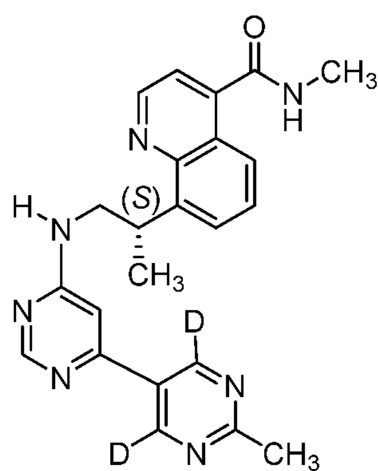
(Compound 1) or
