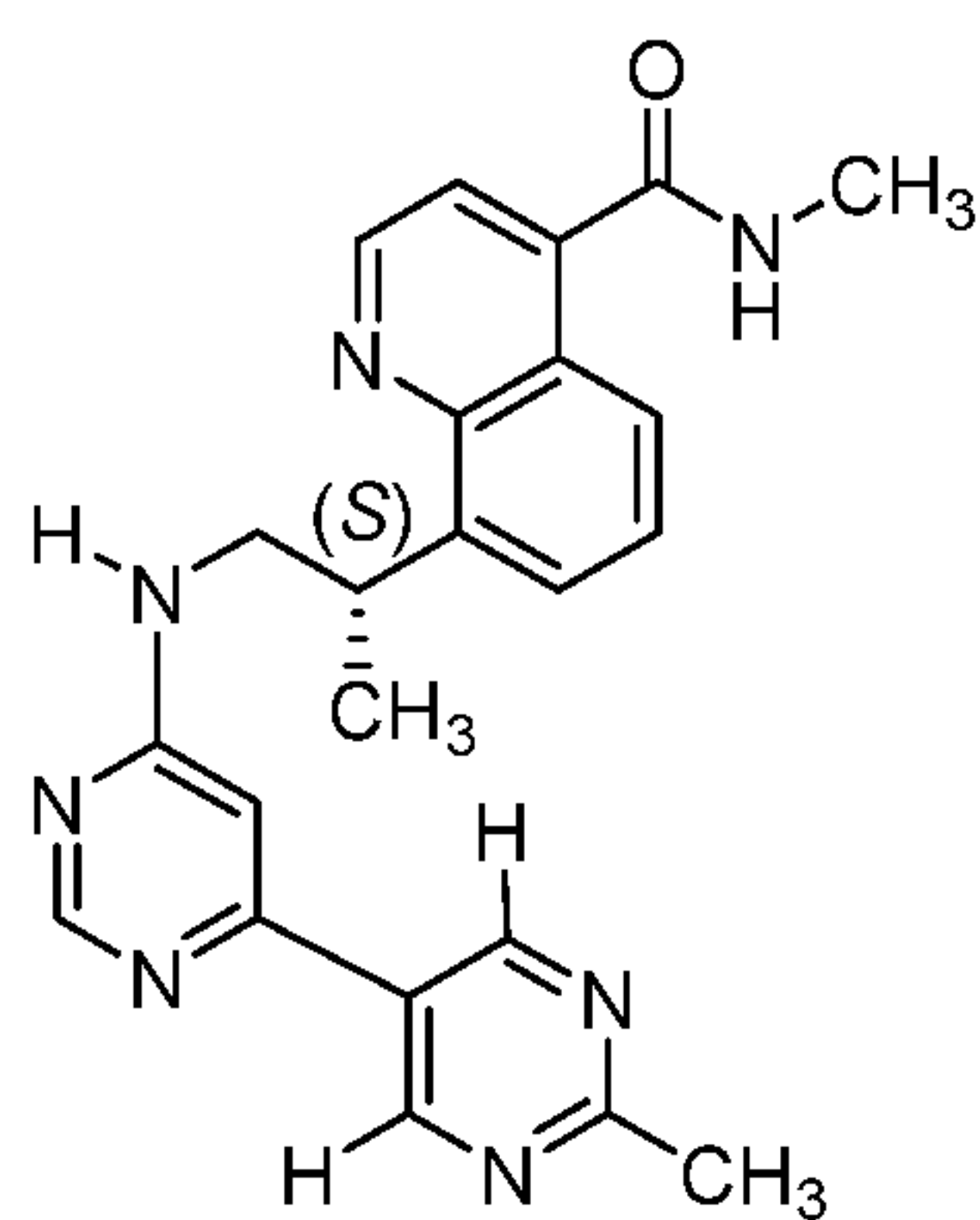
(Compound 1) or
