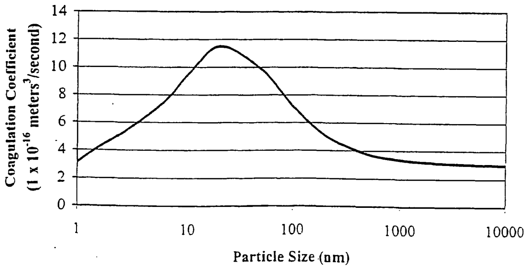
Coagulation Coefficient vs. Particle Size
