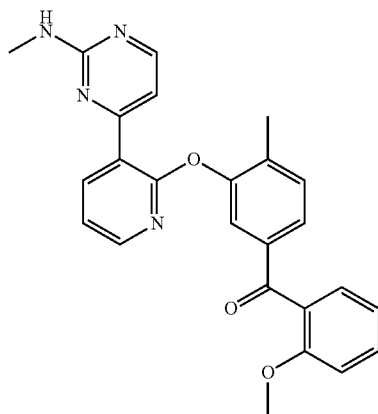
Synthesis of (2-Methoxy-phenyl)-{4-methyl-3-[3-(2-methylamino-pyrimidin-4-yl)-pyridin-2-yloxy]-phenyl}-methanone
