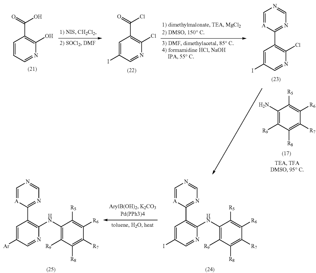
Scheme 8
