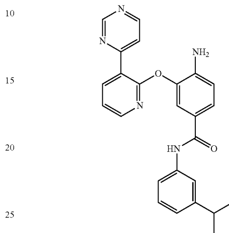
Synthesis of 4-amino-N-(3-isopropylphenyl)-3-(3-(pyrimidin-4-yl)pyridin-2-yloxy)benzamide
