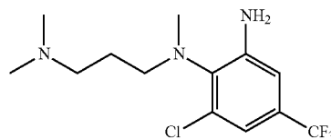
6-chloro-N 1 -(3-(dimethylamino)propyl)-N 1 -methyl-4-(trifluoromethyl)benzene-1,2-diamine
