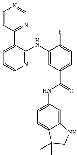
Synthesis of N-(3,3-Dimethyl-2,3-dihydro-1H-indol-6-yl)-4-fluoro-3-(3-pyrimidin-4-yl-pyridin-2-ylamino)-benzamide
