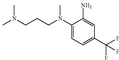
N1-(3-(dimethylamino)propyl)-N1-methyl-4-(trifluoromethyl)benzene-1,2-diamine
