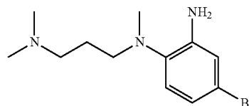
Synthesis of 4-bromo-N1-(3-(dimethylamino)propyl)-N1-methylbenzene-1,2-diamine
