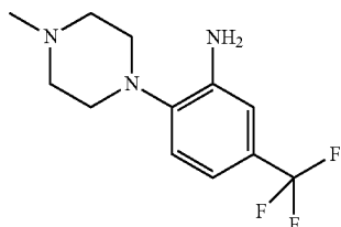
Synthesis of 2-(4-Methyl-piperazin-1-yl)-5-trifluoromethyl-phenylamine
