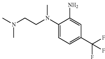
N1-(2-(dimethylamino)ethyl)-N1-methyl-4-(trifluoromethyl)benzene-1,2-diamine
