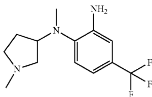
N1-methyl-N1-(1-methylpyrrolidin-3-yl)-4-(trifluoromethyl)benzene-1,2-diamine
