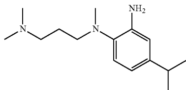
N1-(3-(dimethylamino)propyl)-4-isopropyl-N1-methylbenzene-1,2-diamine
