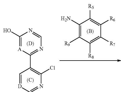
Scheme 7
