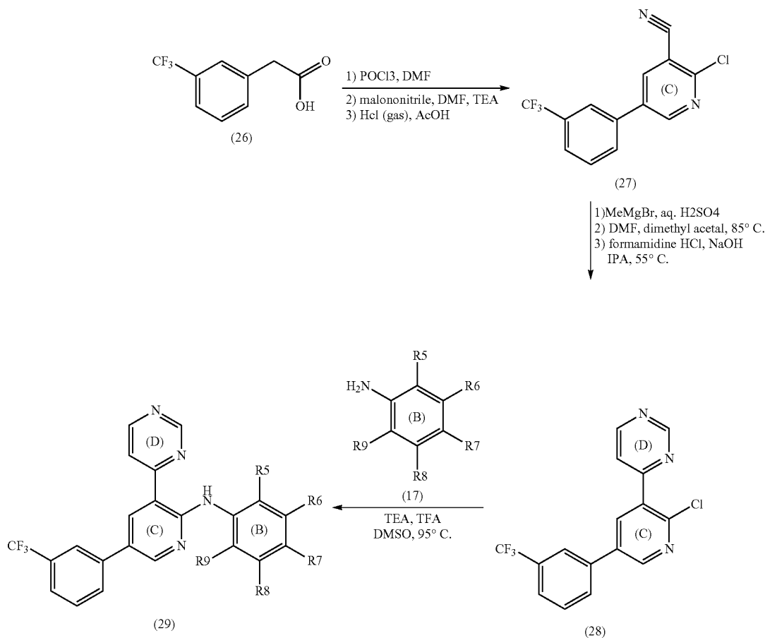
Scheme 9
