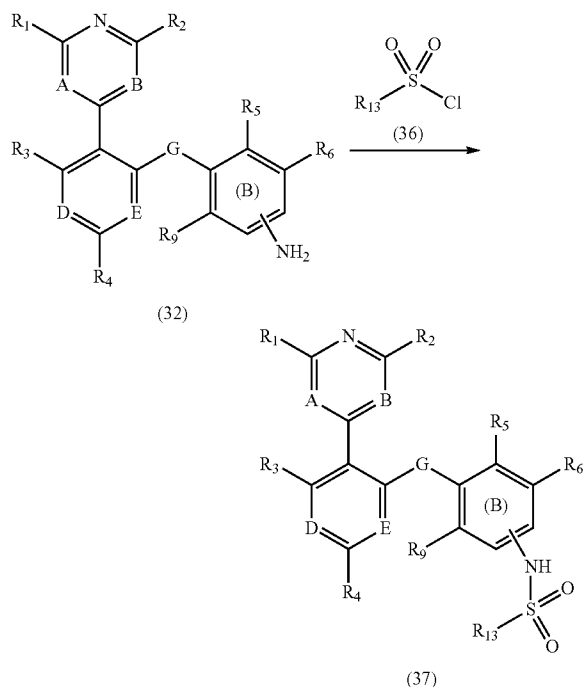
Scheme 13
