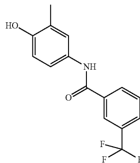
Synthesis of N-(4-hydroxy-3-methylphenyl)-3-(trifluoromethyl)benzamide
