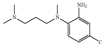
4-chloro-N1-(3-(dimethylamino)propyl)-N1-methylbenzene-1,2-diamine
