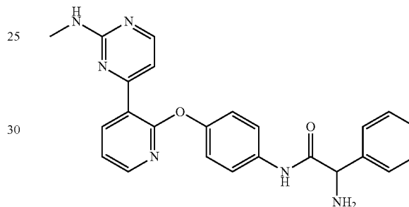
Synthesis of (rac)-2-amino-N-(4-(3-(2-(methylamino)pyrimidin-4-yl)pyridin-2-yloxy)phenyl)-2-phenylacetamide
