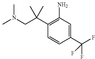
Synthesis of 2-(2-Dimethylamino-1,1-dimethyl-ethyl)-5-trifluoromethyl-phenylamine
