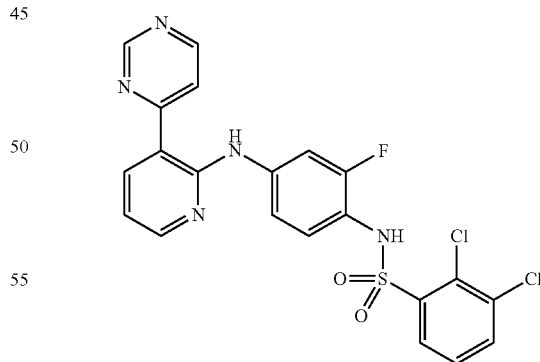
Synthesis of 2,3-dichloro-N-(2-fluoro-4-(3-(pyrimidin-4-yl)pyridin-2-ylamino)phenyl)benzenesulfonamide
