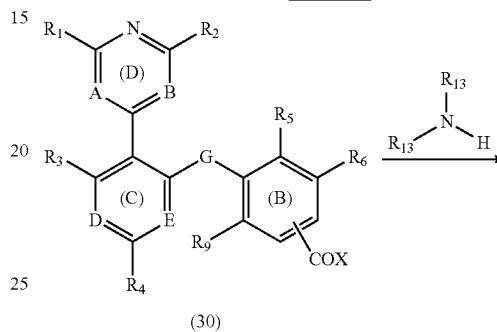
Scheme 10
