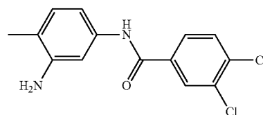
Synthesis of N-(3-amino-4-methyl-phenyl)-3,4-dichloro-benzamide
