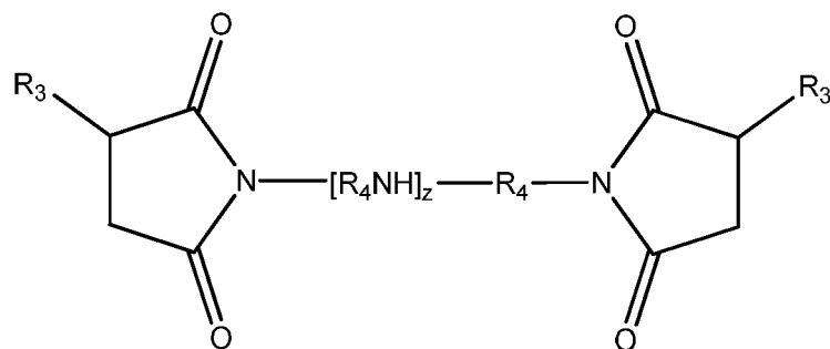
Formula I
