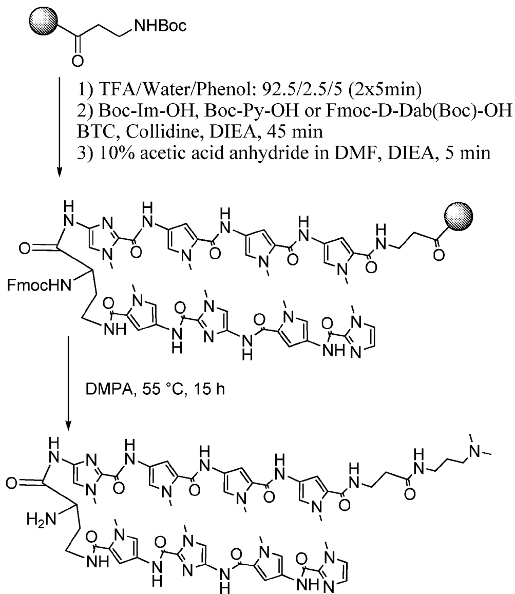
FIGURE 5. Synthesis of Py-Im polyamide on PAM resin
