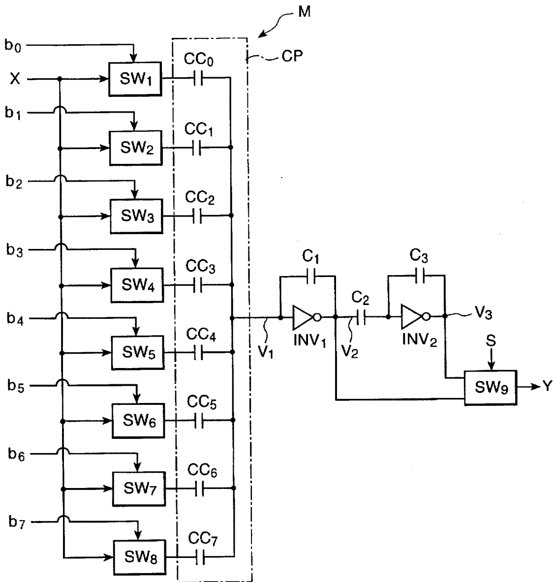
Fig. 2 (PRIOR ART)
