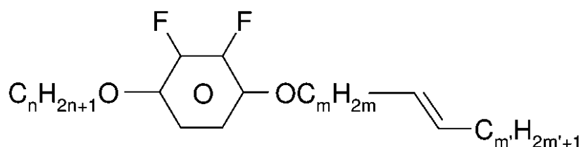
Y-nO-OmVm'
