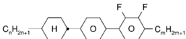
CPY-n-m
