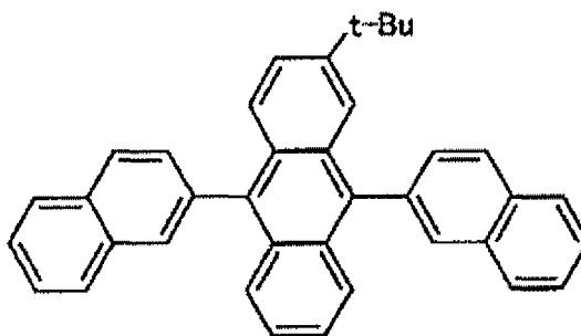
Chemical formula 3
