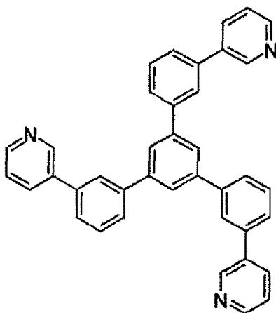
Chemical formula 2
