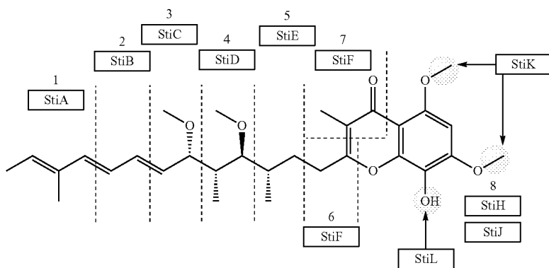
Stigmatellin A
