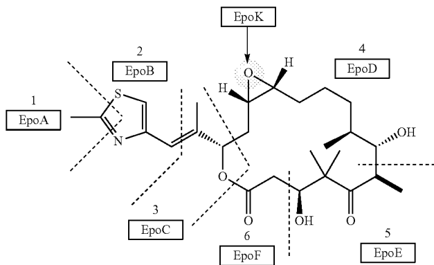
Epothilone A
