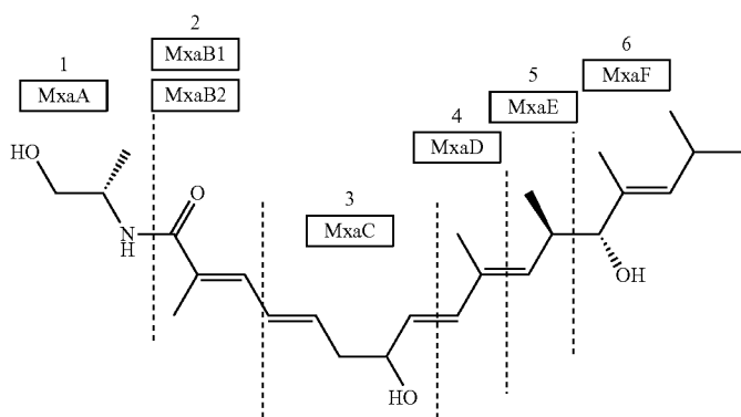
Myralamid S
