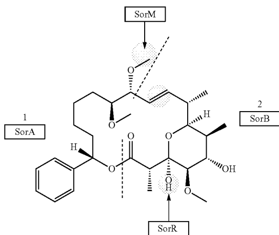
Soraphen A
