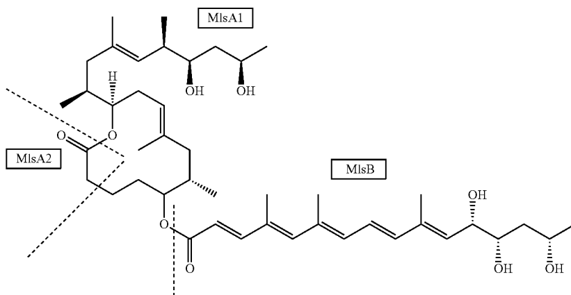
Mycolactone
