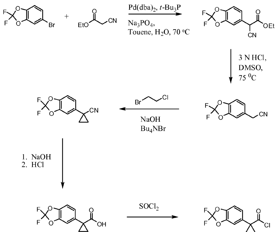
Scheme 2. Alternative synthesis of the acid chloride moiety.
