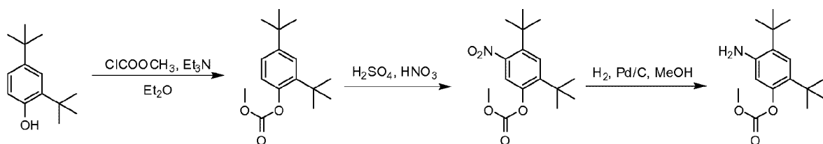
Scheme 6: Synthesis of the amine moiety.
