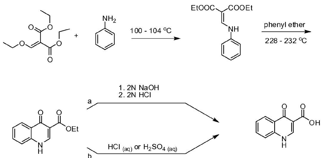
Scheme 6: Synthesis of the amine moiety.
