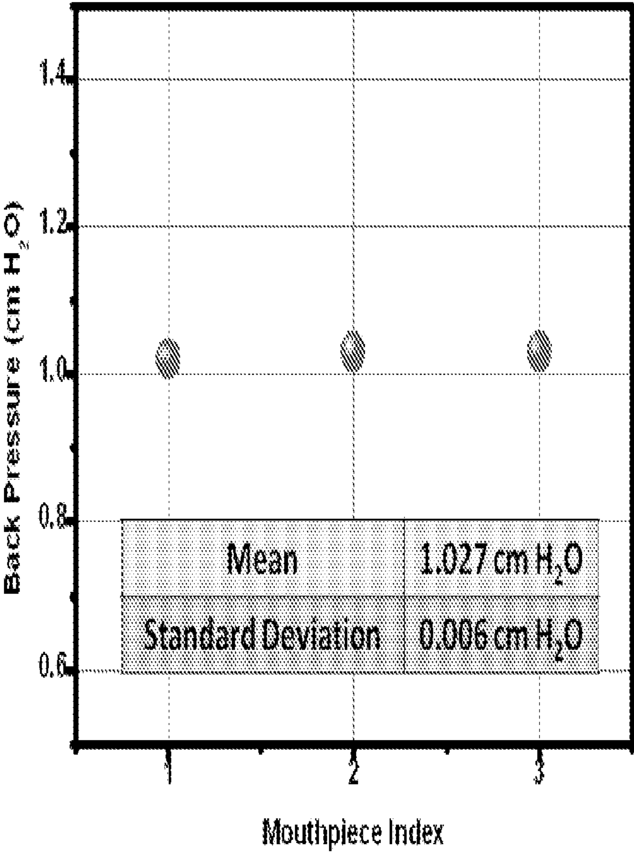
Typical back pressure of the mouthpiece
