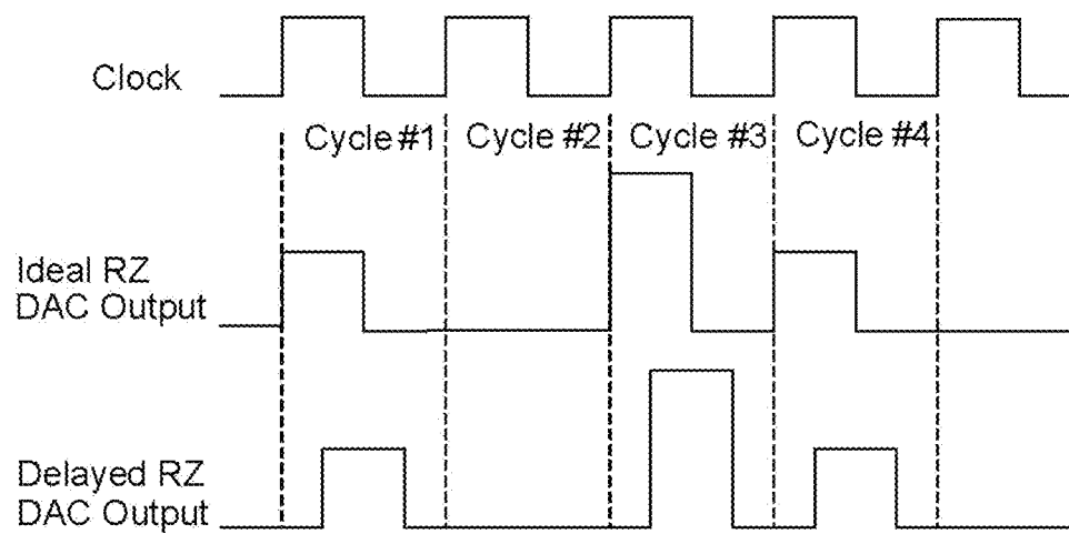
(a) RZ CT DAC
