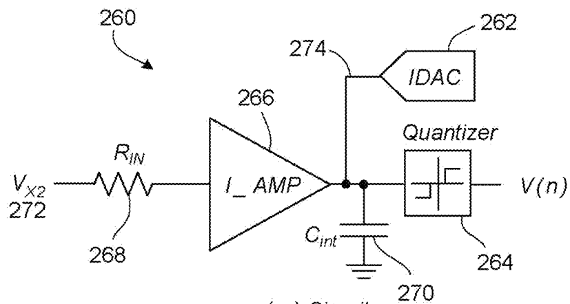
(a) Circuit
