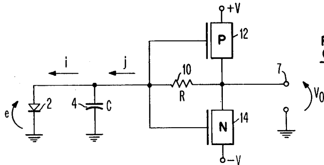
RESISTOR SHUNT CMOS AMPLIFIER
