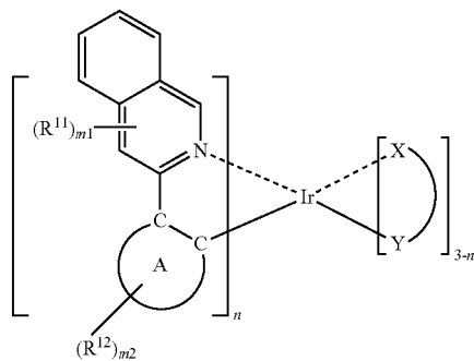
General Formula (3)
