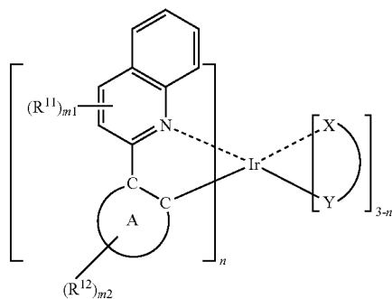
General Formula (2)
