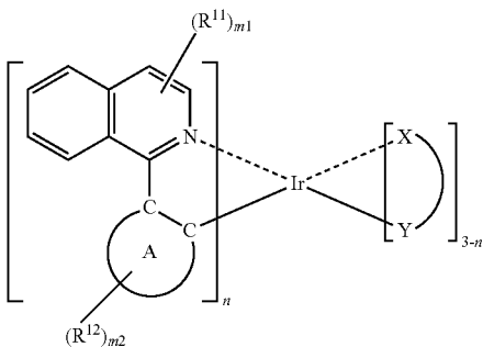
General Formula (3)
