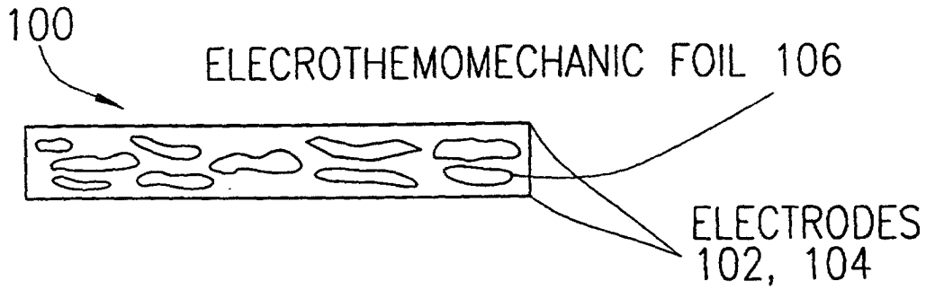
FIG. 3a (THE EMF TECHNOLOGY)
