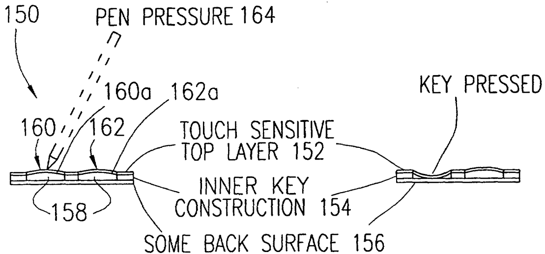
FIG. 4c (KEY CONSTRUCTION NO.3)
