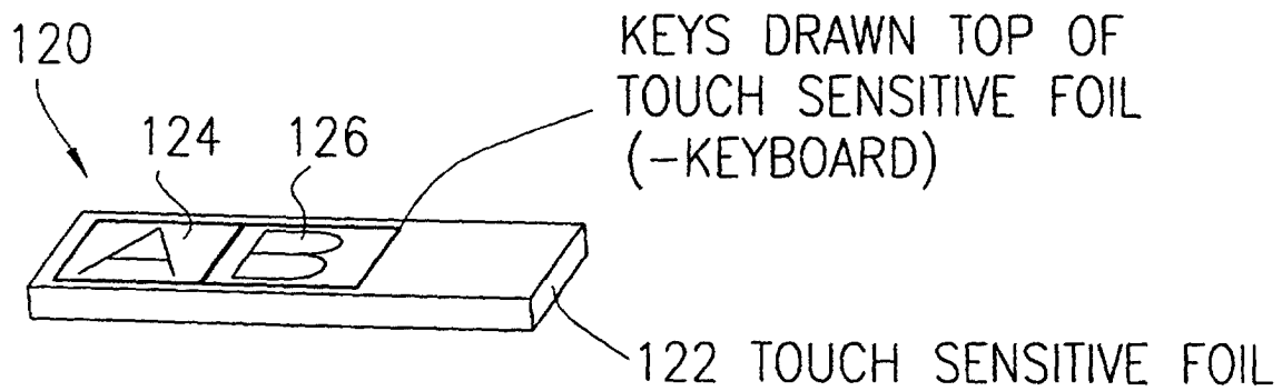
FIG. 4a (KEY CONSTRUCTION NO.1)
