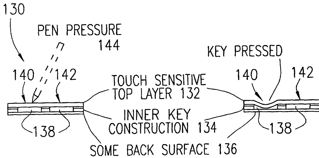
FIG. 4b (KEY CONSTRUCTION NO.2)
