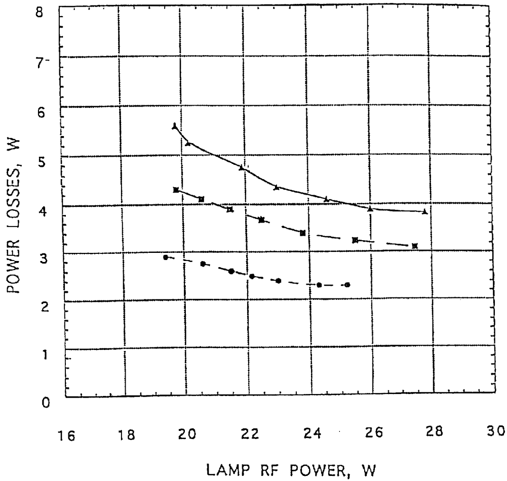
FIG. 6 COIL/FERRITE POWER LOSSES vs LAMP POWER
