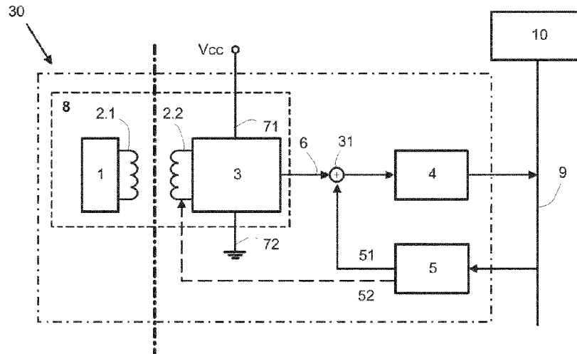
1 CODE-BEARING ELEMENT 3 CODE-READING ELEMENT 4/5 MICROPROCESSOR 8 SENSOR 10 CONTROL UNIT 30 BUS NODE
