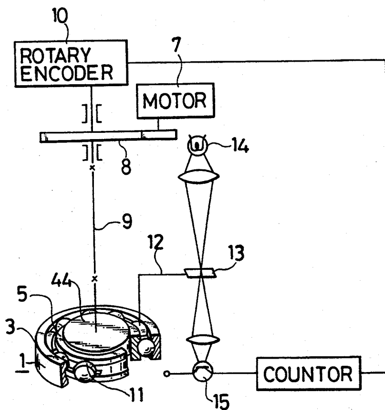
FIG. 6 PRIOR ART
