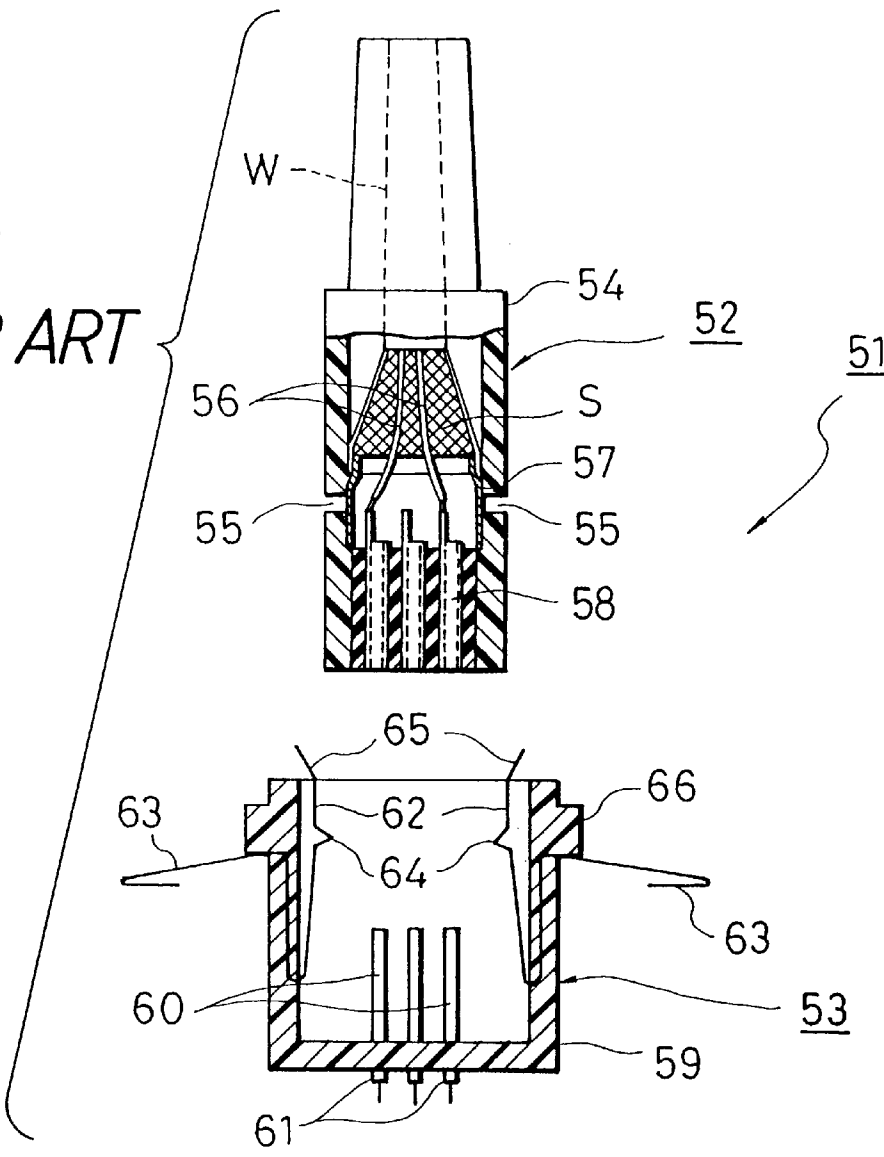
FIG. 8 PRIOR ART
