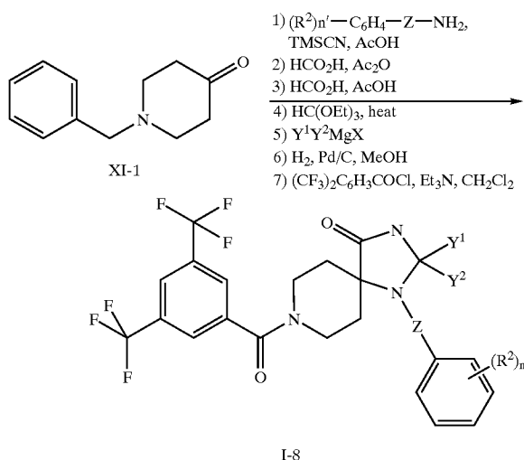
Scheme 12
