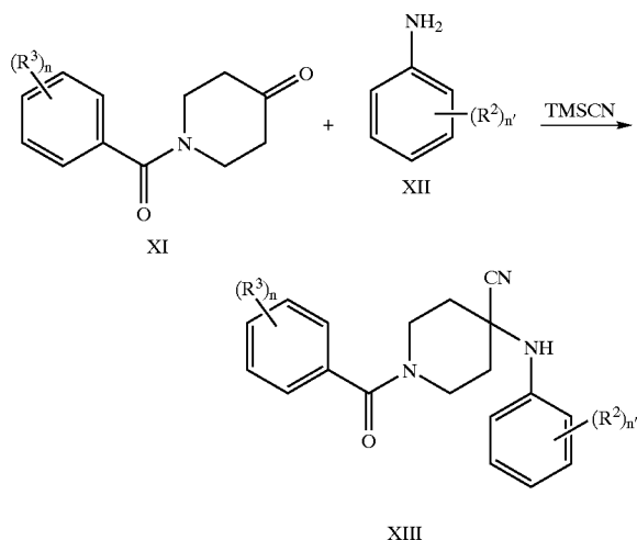
Scheme 11 (intermediates)
