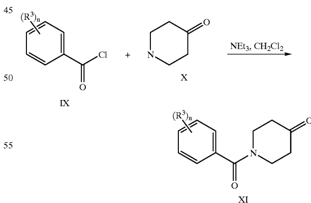
Scheme 10 (intermediates)
