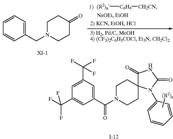
Scheme 16
