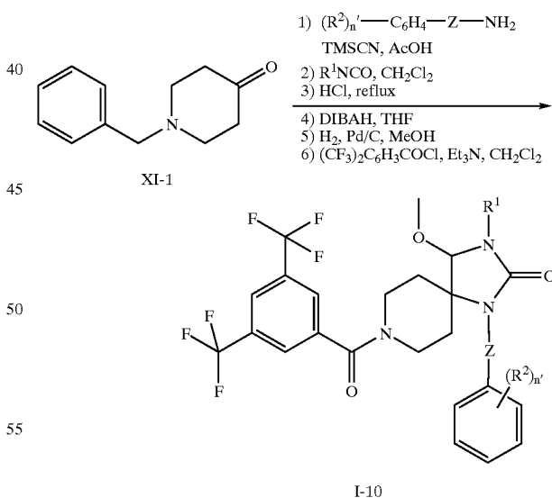
Scheme 14
