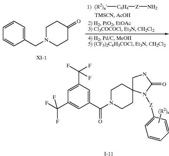
Scheme 15
