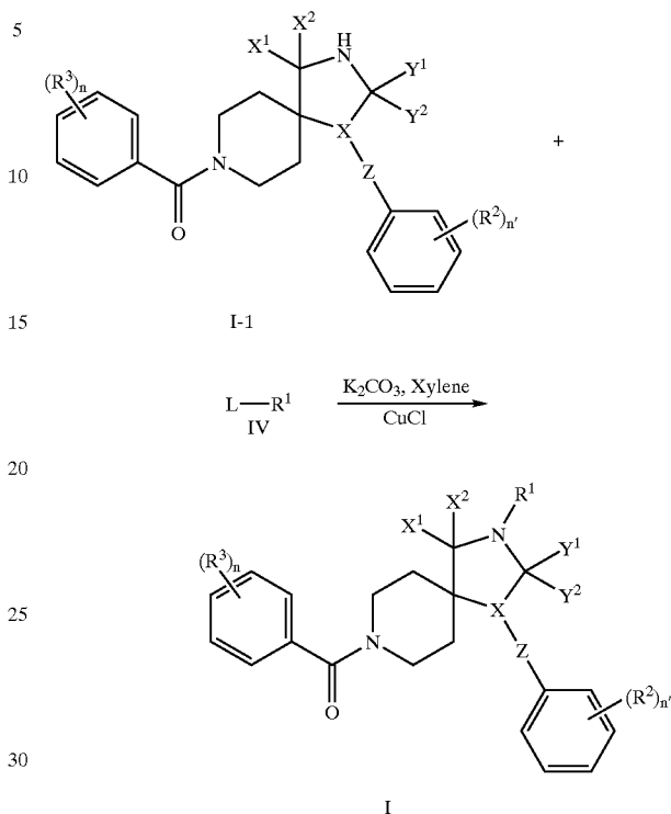
Scheme 6
