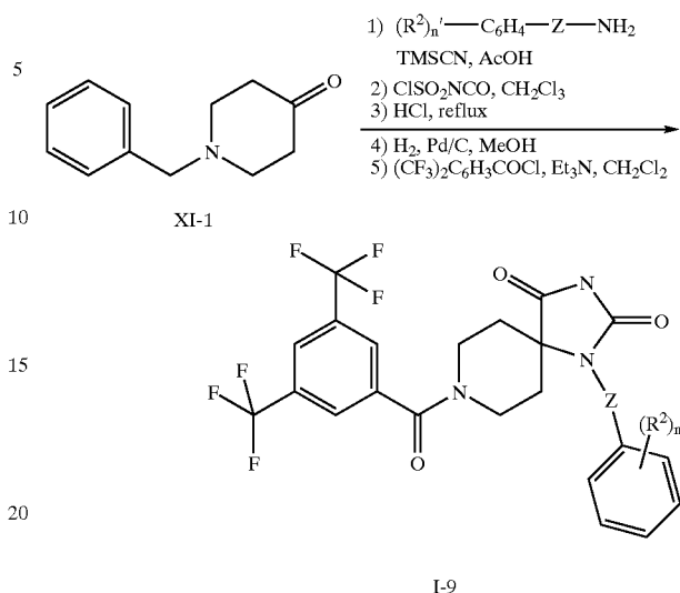
Scheme 13
