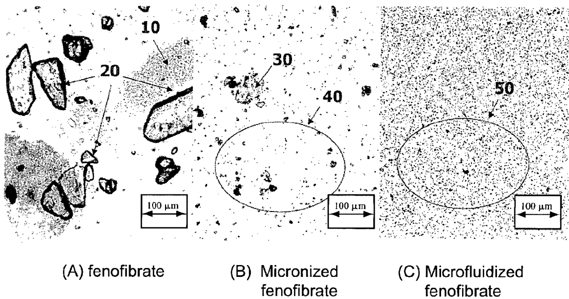
Fig. 1 Optical microscopic comparison of microfluidized fenofibrate with micronized fenofibrate and fenofibrate
