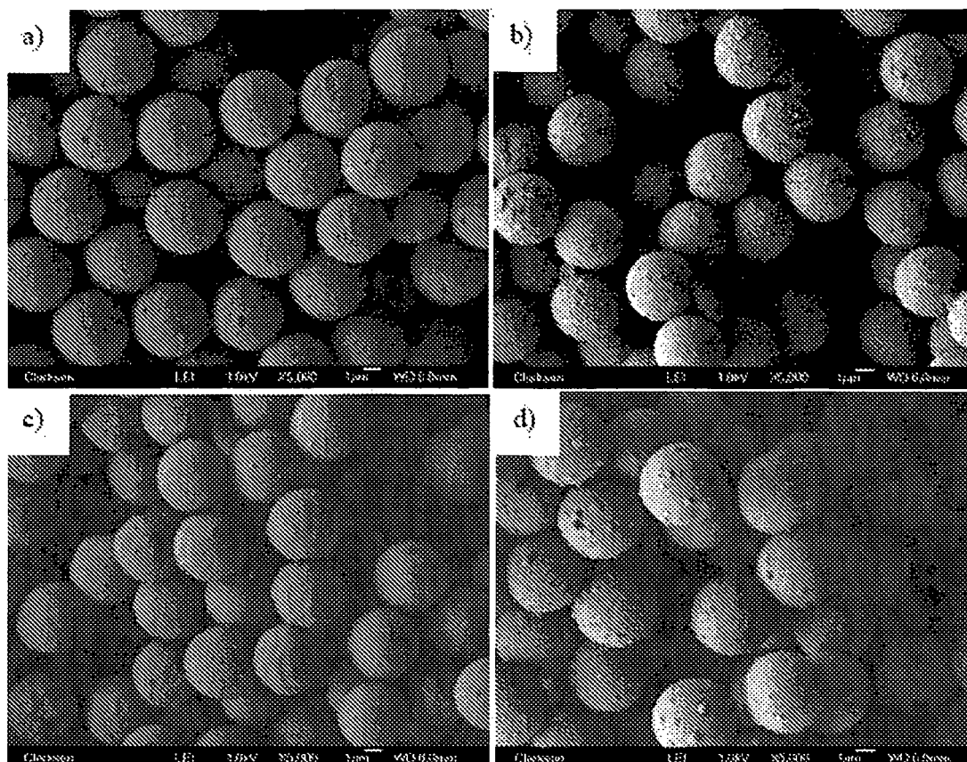
Figure 9. FE-SEM images of Nickel coated polymer particles with a varying Ni layer thickness: a) 40 nm, b) 80 nm c) 100 nm, and d) 120 nm (Samples 5-8, Table 2) (Note: the nominal diameter of the polymer spheres is 3.8 \mu\text{m} ).
