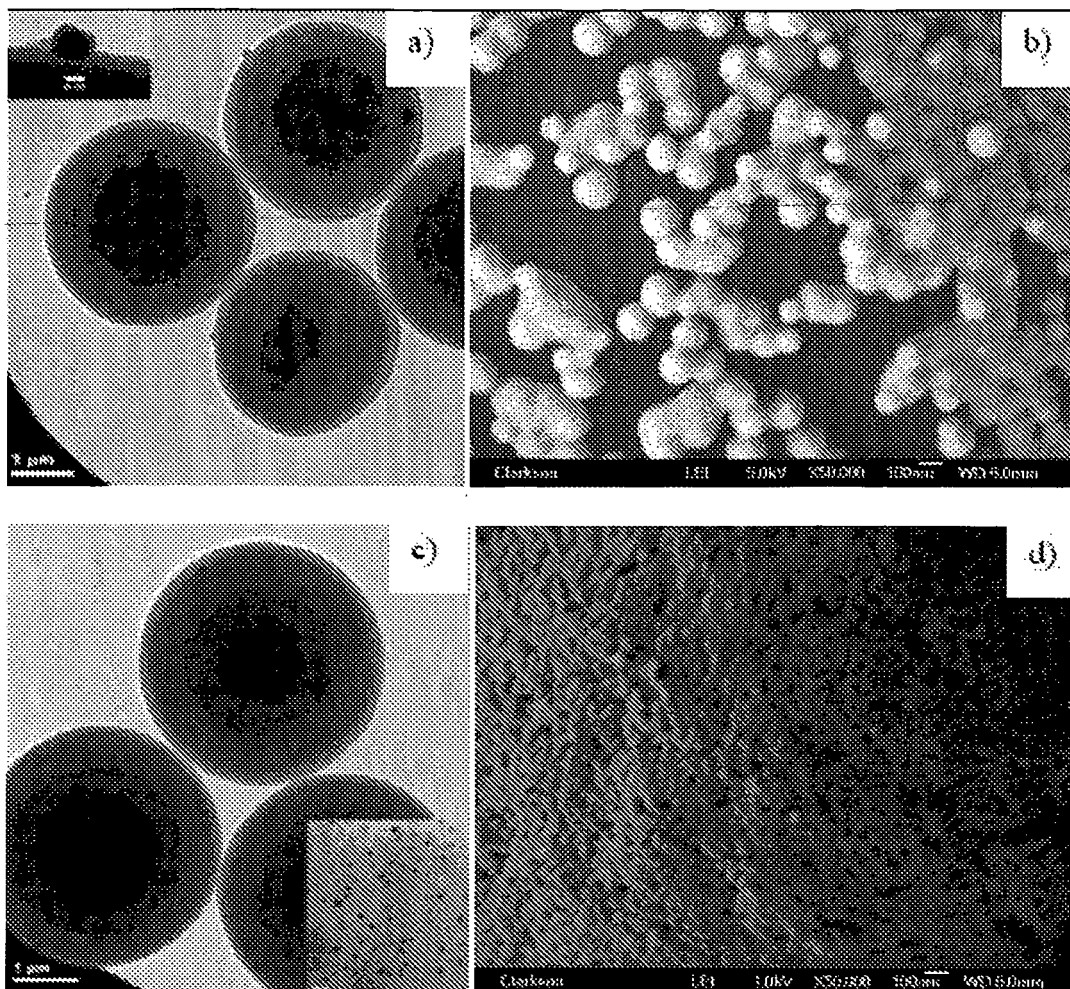
Figure 2. a) TEM image of Pd coated polymer particles conditioned in EDA for 22 hrs (the inset shows the image of a large Pd cluster), b) high magnification FESEM of the surface of a polymer particle shown in (a) coated with nickel, c) TEM image of a Pd coated polymer sphere conditioned in TEPA for 96 hours, and d) FESEM of a polymer particle shown in (c) coated with nickel. (Note: Nominal diameter of the polymer spheres is 3.8 \mu\text{m} ).
