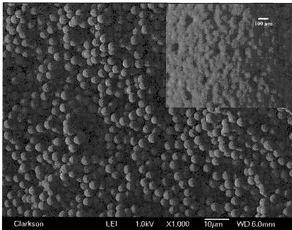
Figure 7. Electron micrograph of Nickel coated polymer particle with 40% GMA content. Inset shows high magnification of the surface of a single particle.
