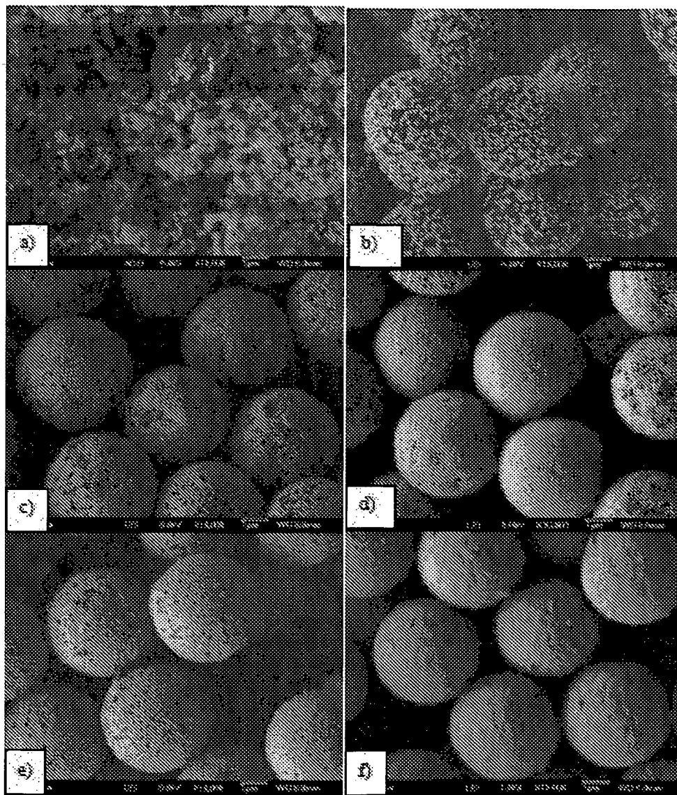
Figure 1. FESEM images of Nickel coated polymer particles: (a) not conditioned with amine; conditioned for 22 hours with (b) EDA, (c) DETA, (d) TETA and (e) TEPA; and (f) conditioned for 96 hours with TEPA (Note: the nominal diameter of the polymer spheres is 3.8 \mu\text{m} ).
