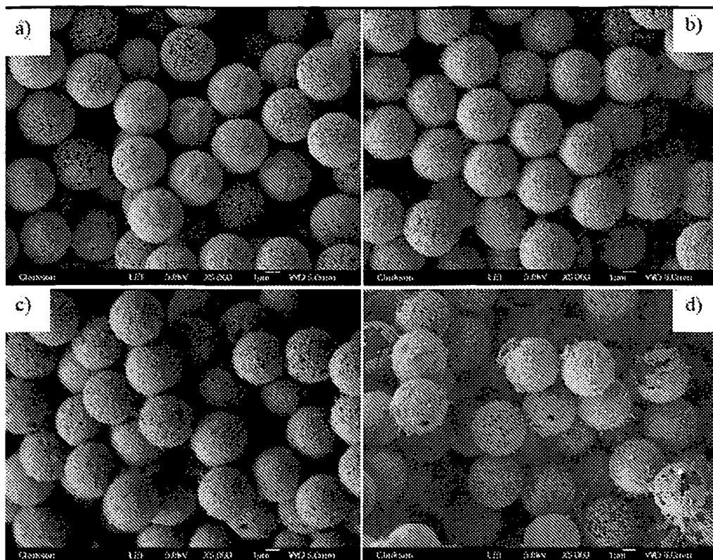
Figure 8. FE-SEM images obtained using different \text{NH}_3 :Ni molar ratios: (a) 2:1; (b) 2.5:1; (c) 3.5:1; and (d) 6:1 (Samples 1-4, Table 2) (Note: the nominal diameter of the polymer spheres is 3.8\ \mu\text{m} ).
