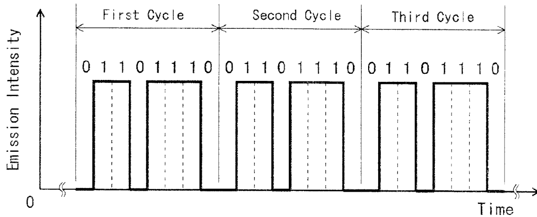
(B) Blinking Pattern of Light Source
