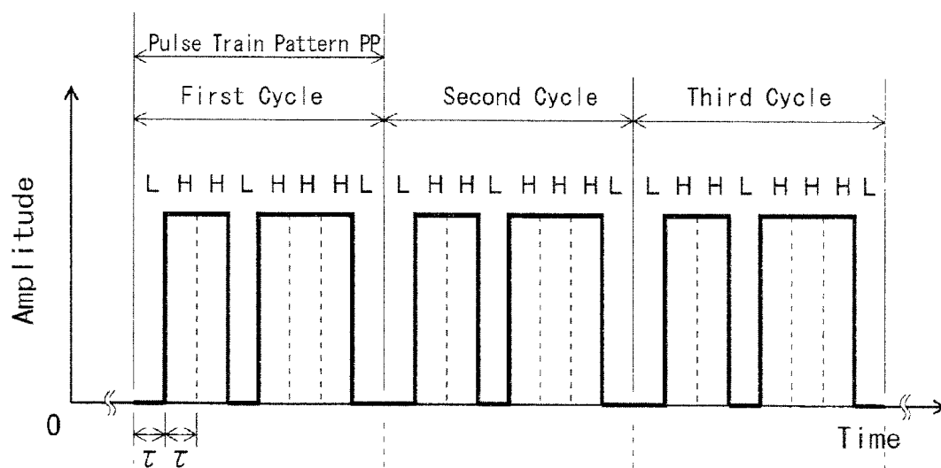
(A) Control Pulse Signal CS
