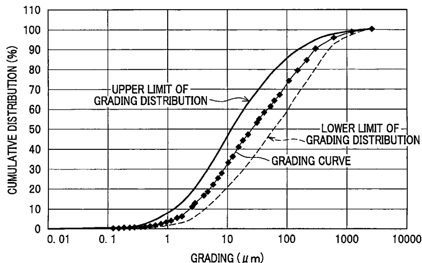
CUMULATIVE GRADING CURVE OF POWDER
