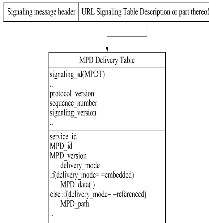
MPD Delivery Table Description Semantics
