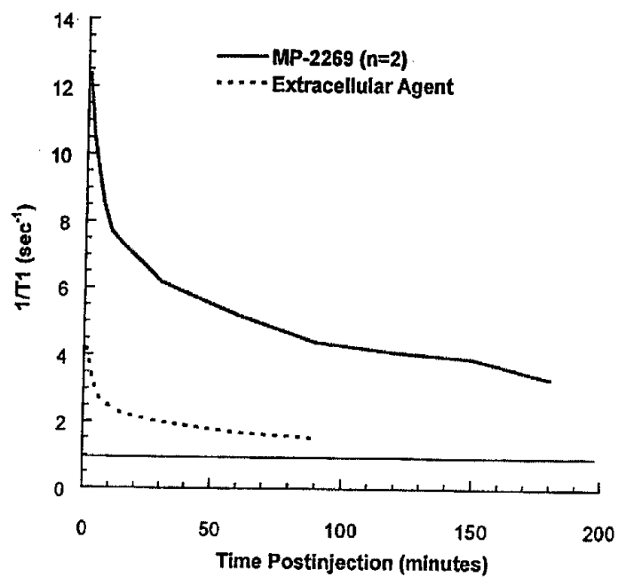
Figure 1. T1 (1/T1) vs. Time Postinjection of a Single Bolus (45 \mu\text{mol/kg} ) of Gadolinium(III)-4-pentylbicyclo[2.2.2]octane-1-carboxyl-L-aspartyl-L-aspartyl-4-aminobutyldiethylenetriaminepentaacetic acid (MP-2269) in a Rabbit.
