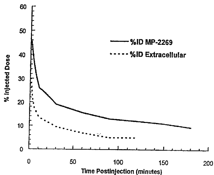
Figure 2. % Injected Dose (ID) vs. Time Postinjection of a Single Bolus ( 45 \mu\text{mol/kg} ) of Gadolinium(III)-4-pentylbicyclo[2.2.2]octane-1-carboxyl-L-aspartyl-L-aspartyl-4-aminobutyldiethylenetriaminepentaacetic acid in a Rabbit.
