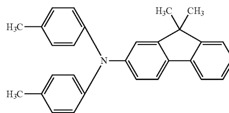
Structural formula (11)
