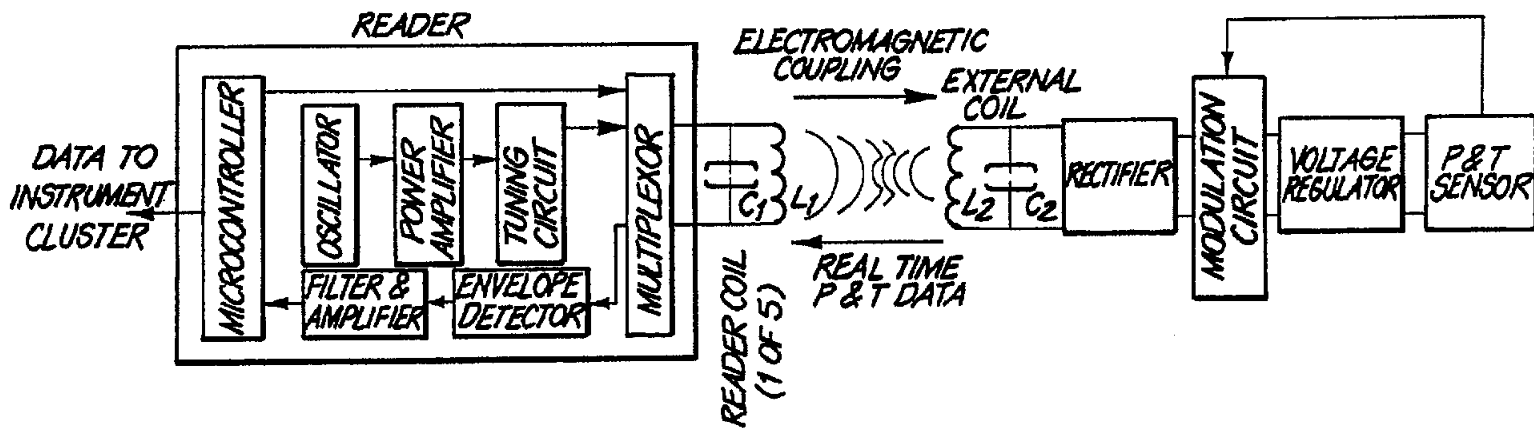
SYSTEM BLOCK DIAGRAM
