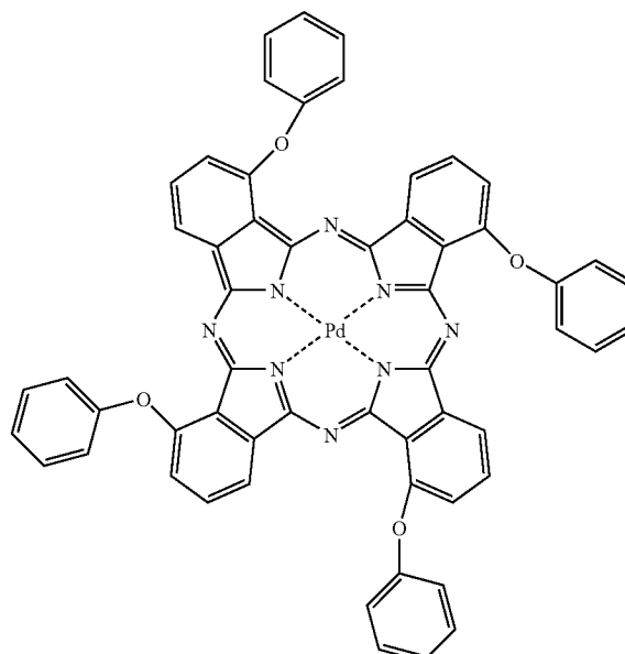
Exact Mass: 986.16 gmol -1
