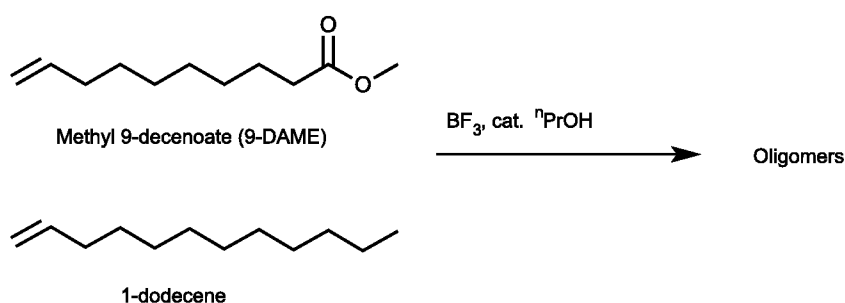
Scheme 1. BF 3 -mediated co-oligomerization of methyl 9-decenoate and 1-dodecene.
