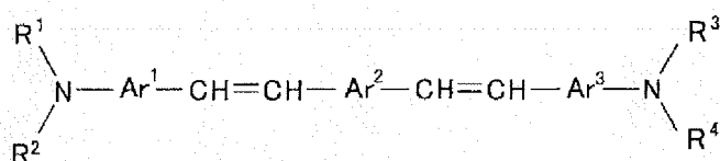
Structural Formula (1)
