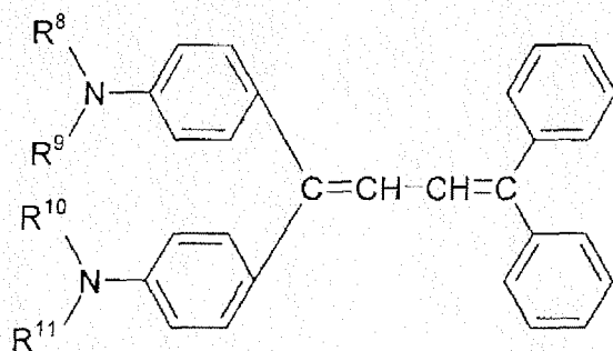
Structural Formula (3)
