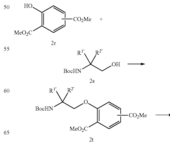
Scheme 4. General synthesis of amides described in the disclosure.
