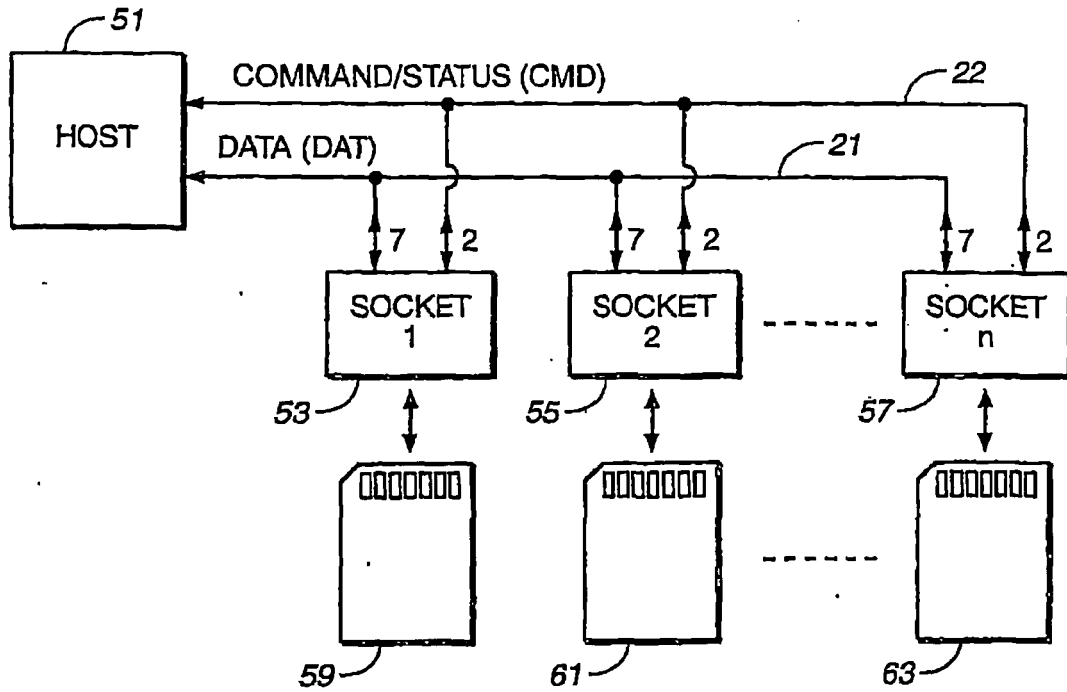
FIG. 3 (PRIOR ART)
