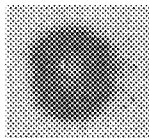
FUNDAMENTAL PARTICLE
