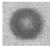
2 PARTICLES COALESCED
