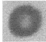
3 PARTICLES COALESCED
