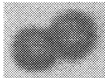
2 PARTICLES COMBINED
