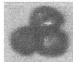
3 PARTICLES COMBINED
