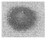
FUNDAMENTAL PARTICLE
