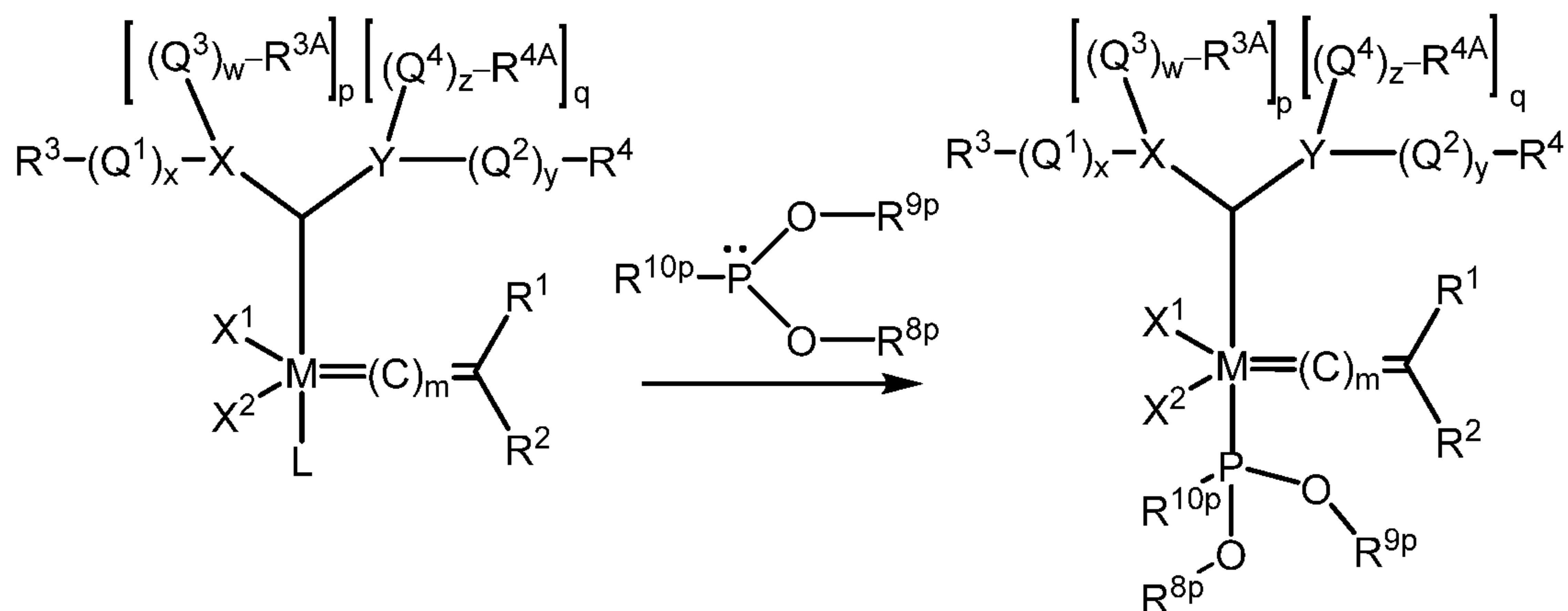
Formula (IIIS)
