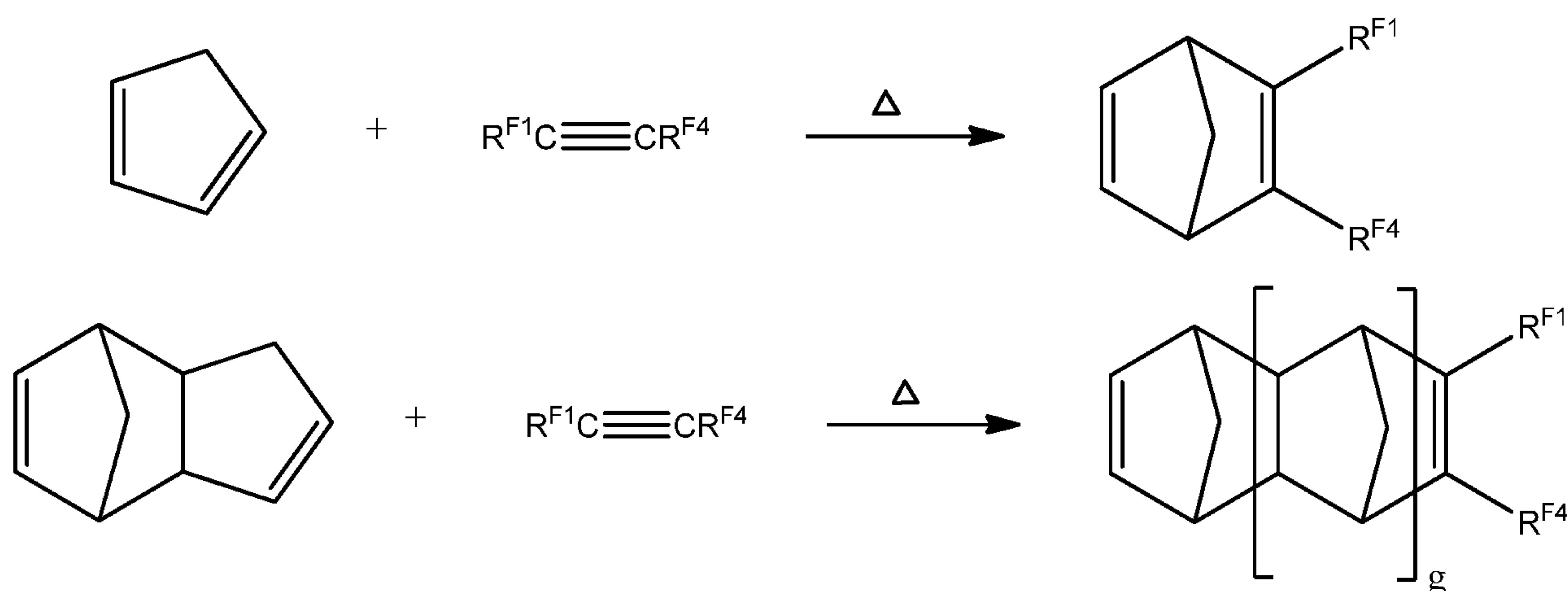
SCHEME 6
