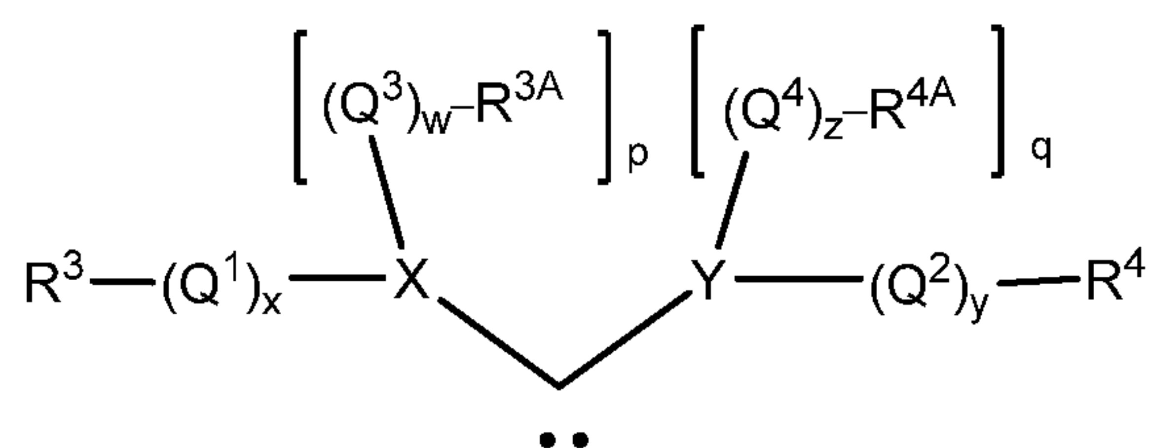
Formula (II)
