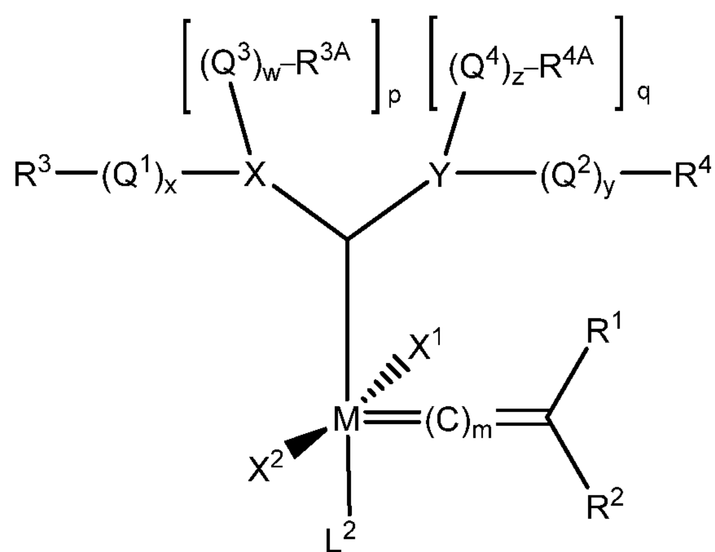
Formula (IIIa)
