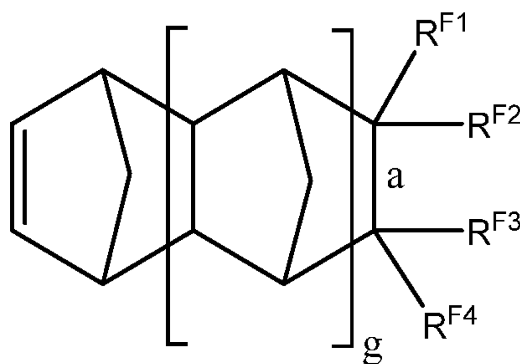
Formula (F)
