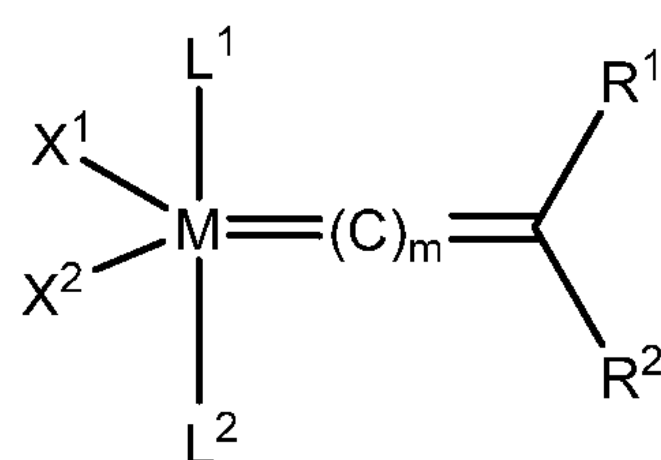
Formula (I)
