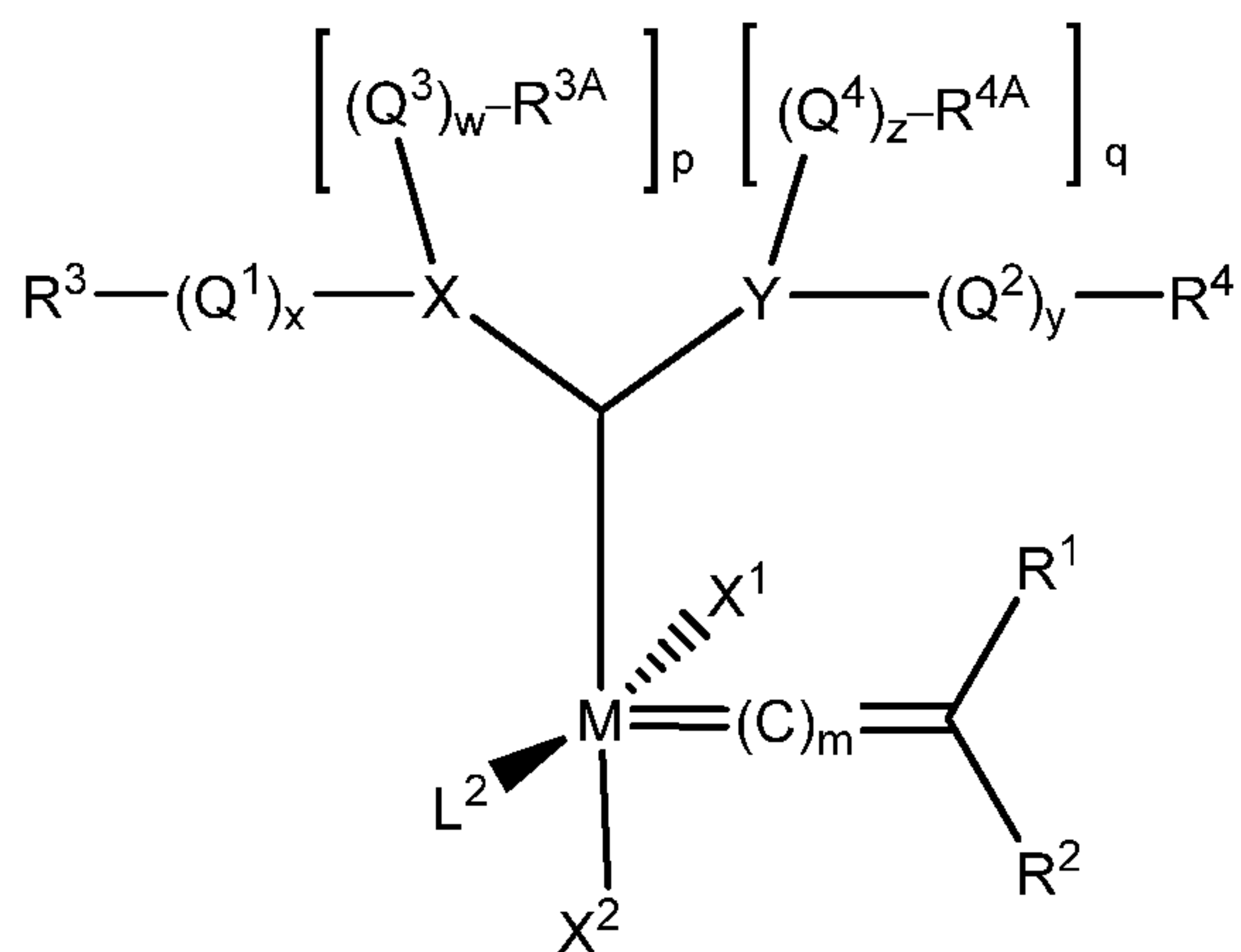
Formula (IIIb)
