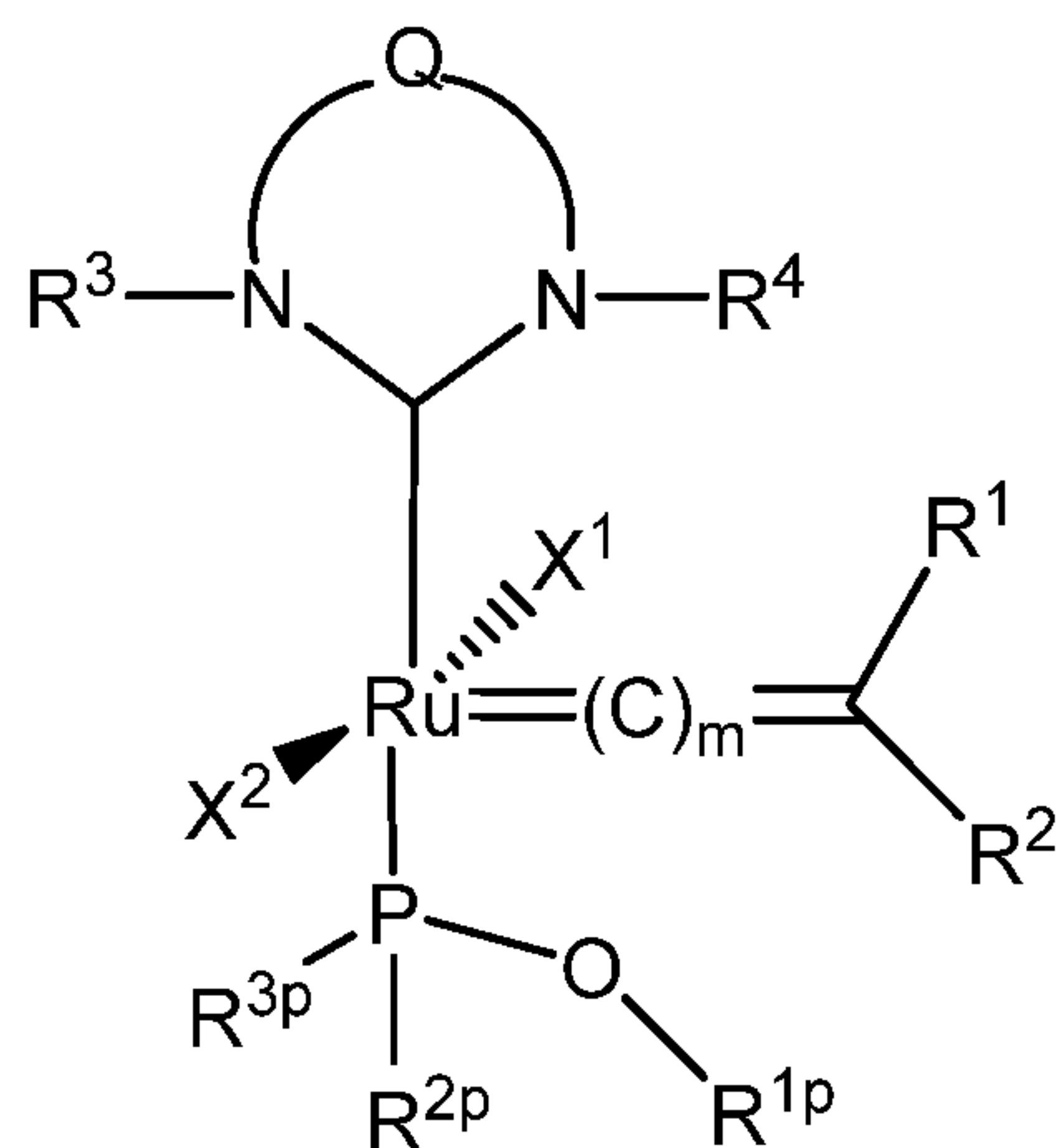
Formula (VIa)
