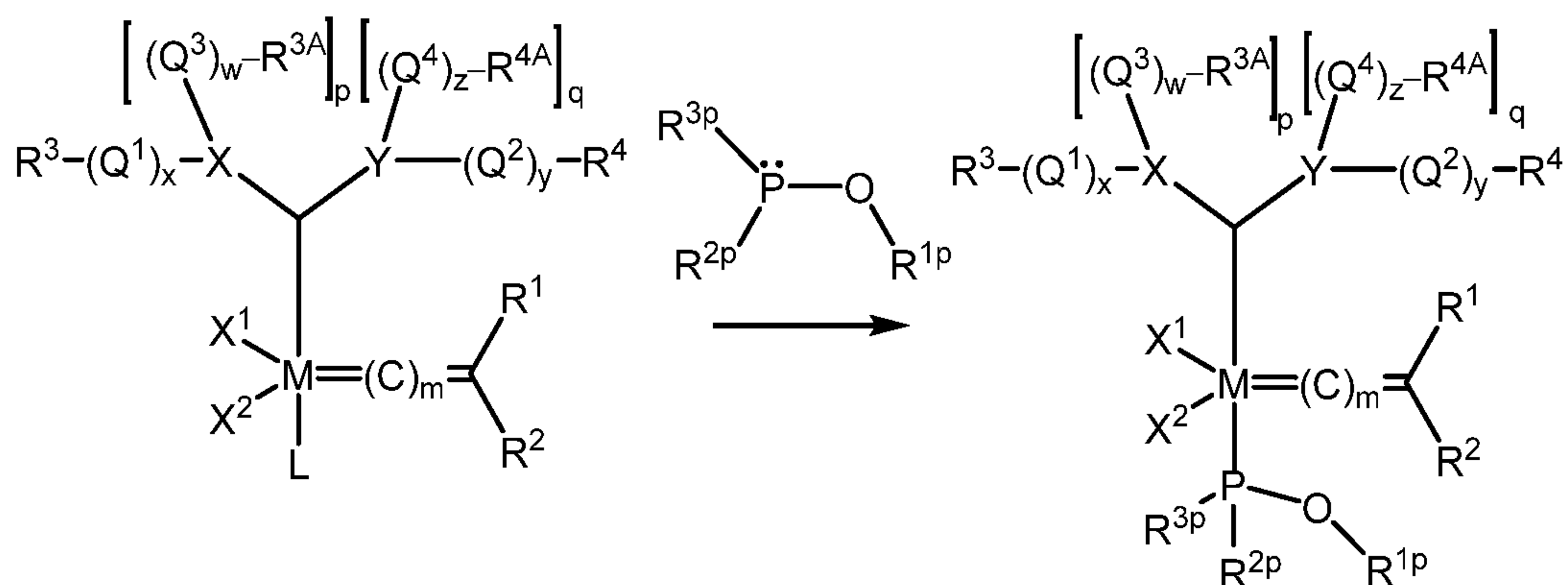
Formula (IIIS)
