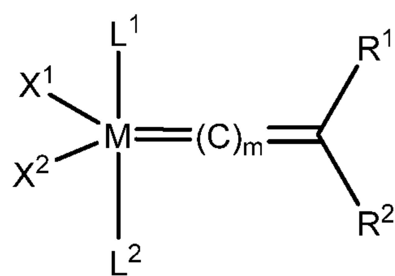
Formula (I)
