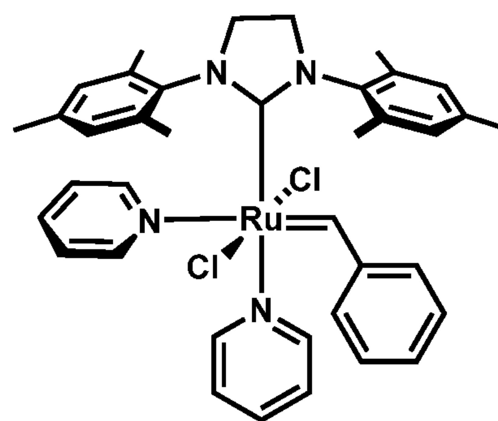
trans C727
