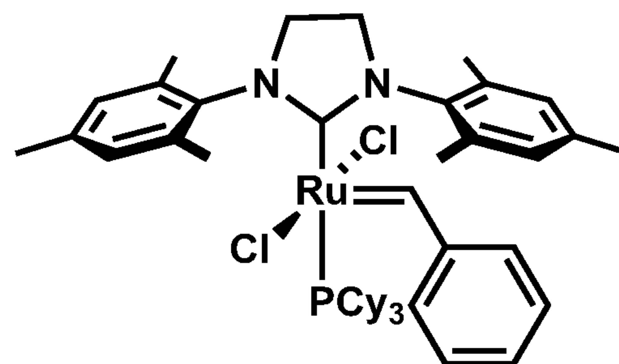
trans-C848
