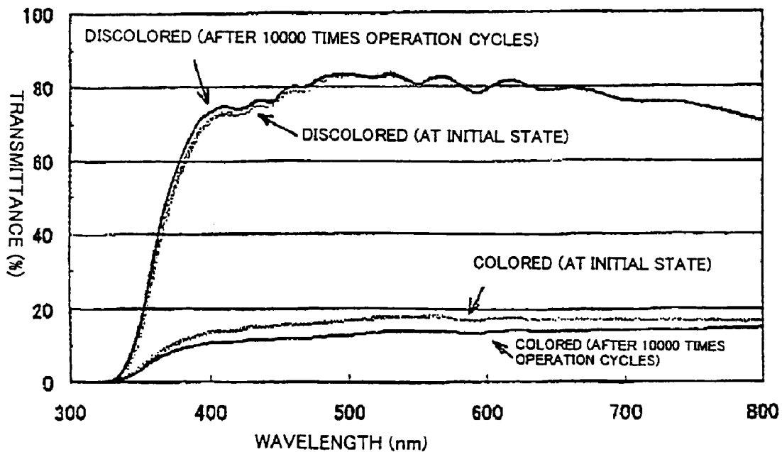
SPECTRAL OF PRESENT SAMPLE A (HAVING INTERMEDIATE LAYER OF SnO 2 .)
