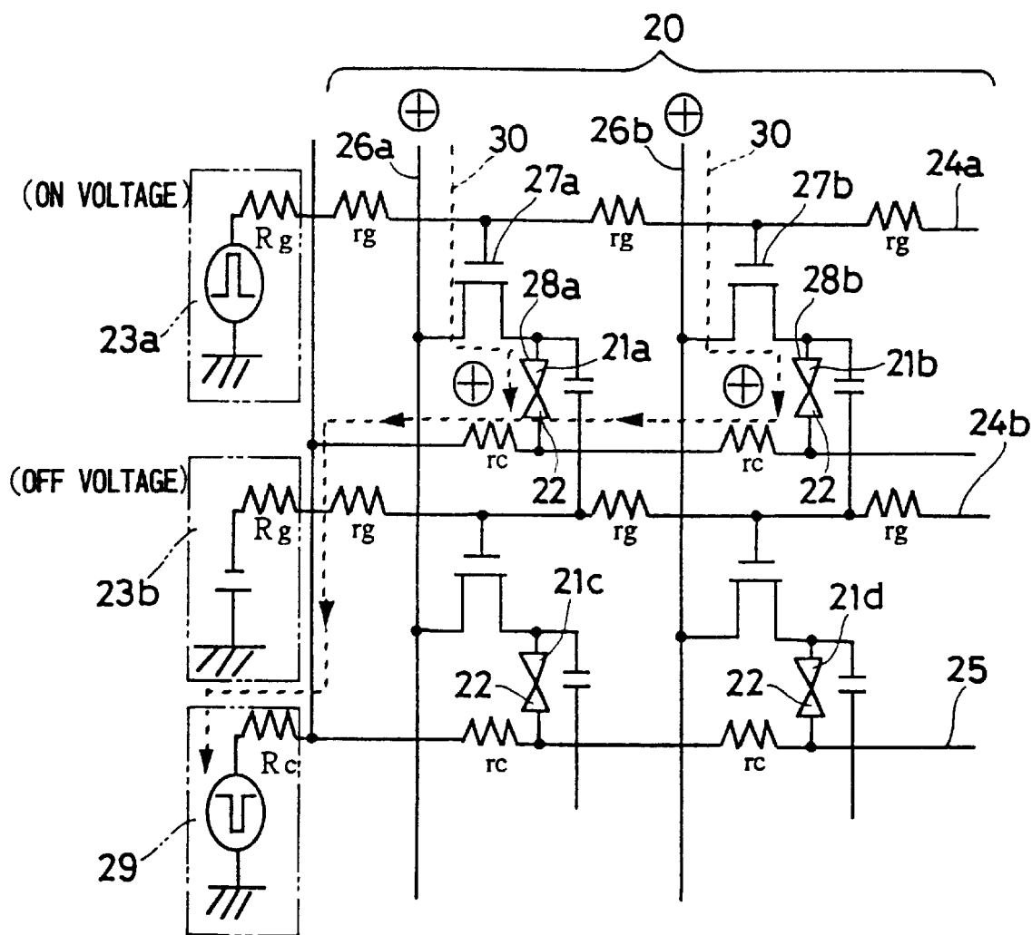
FIG. 14 PRIOR ART
