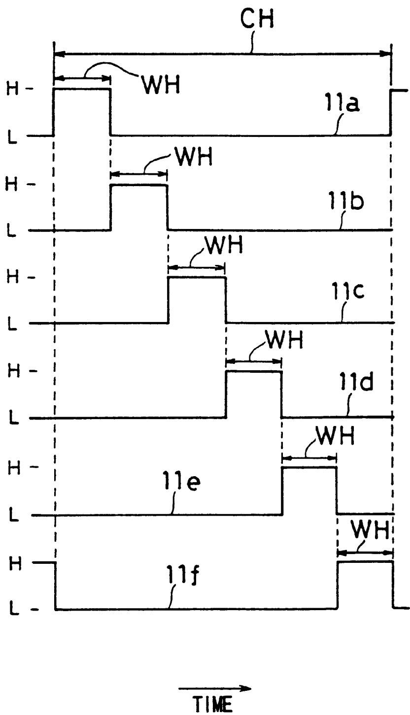
FIG. 11 PRIOR ART
