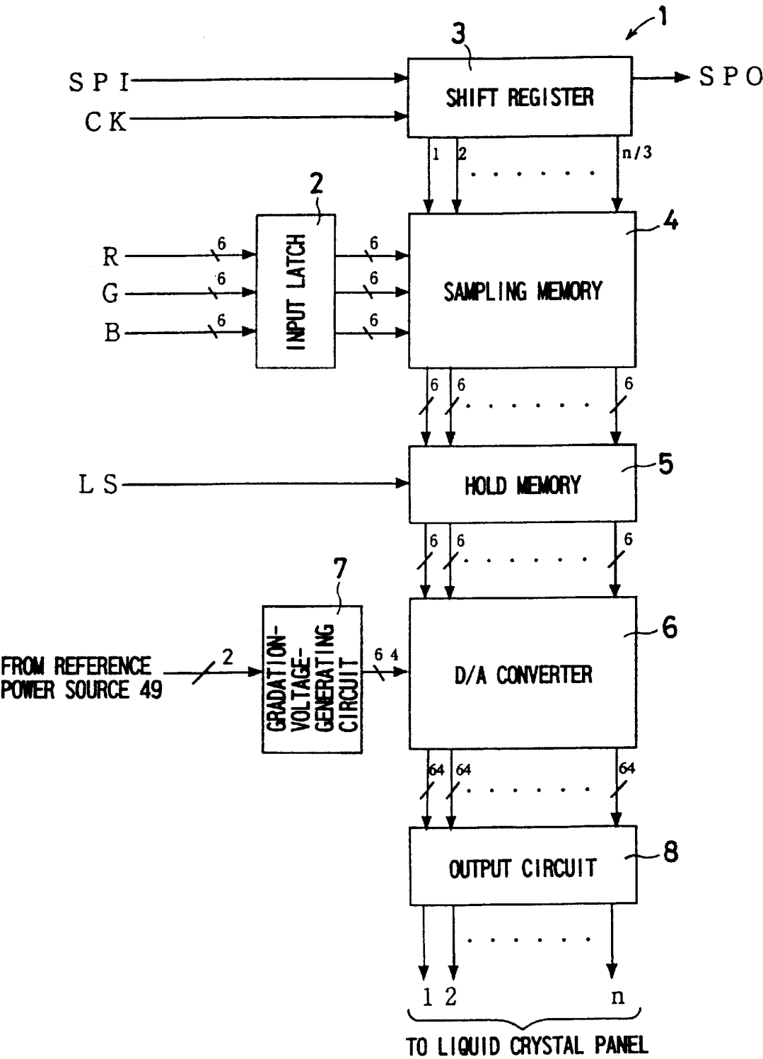
FIG. 10 PRIOR ART
