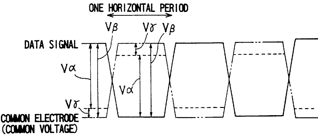
FIG. 15 PRIOR ART
