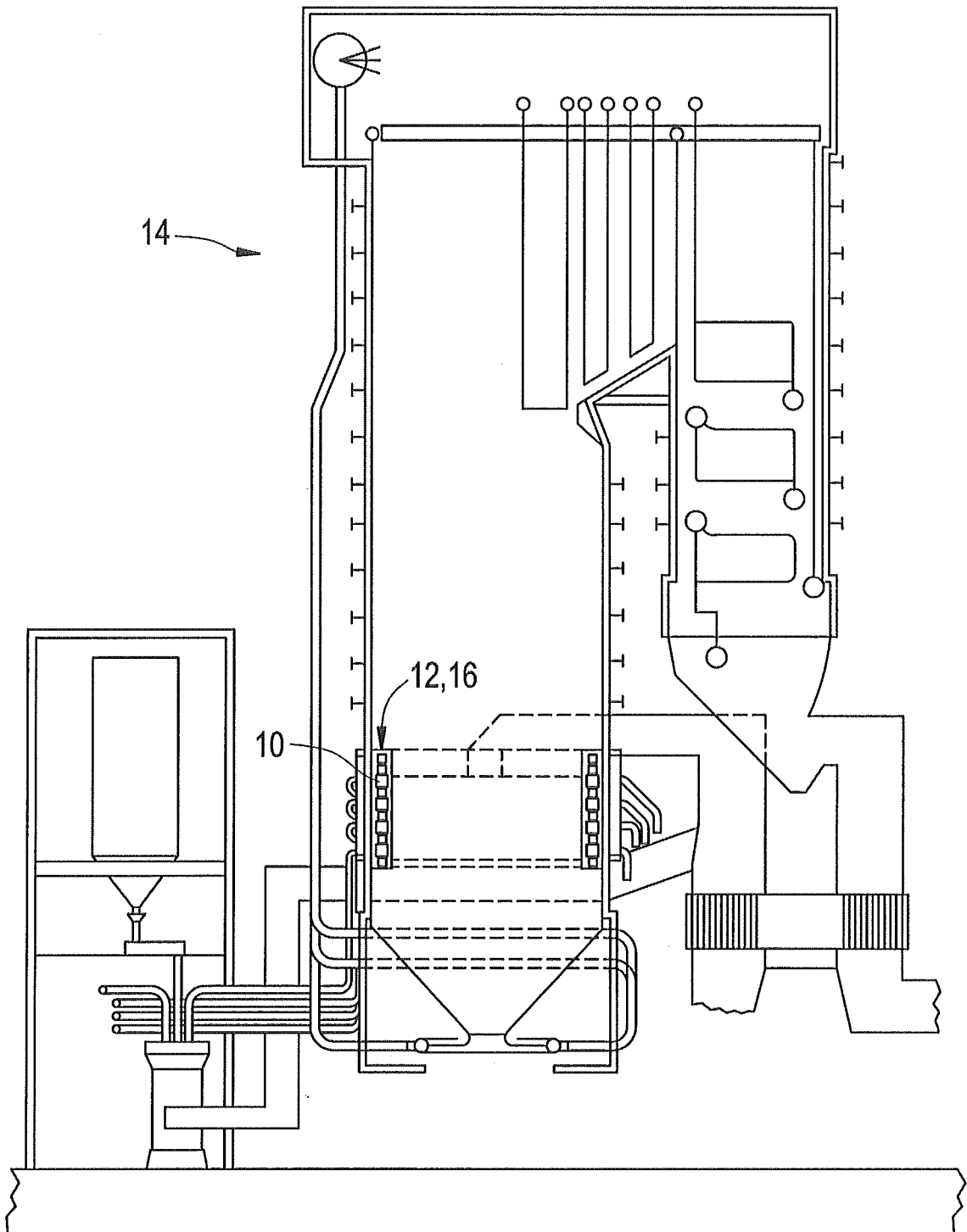
FIG. 1 Prior Art
