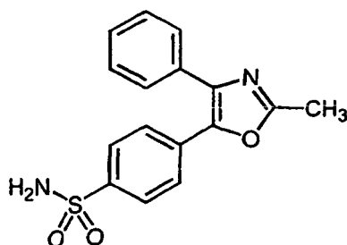
4-(2-methyl-4-phenyl-5-oxazolyl)benzenesulfonamide; C13)
