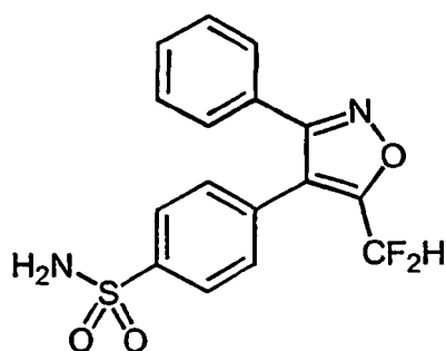
4-[5-(difluoromethyl)-3-phenylisoxazol-4-yl]benzenesulfonamide; C25)
