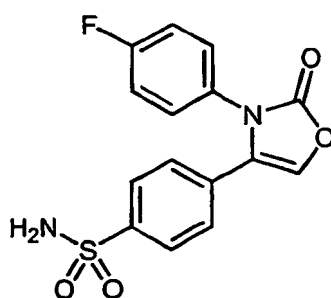
4-[3-(4-fluorophenyl)-2,3-dihydro-2-oxo-4-oxazolyl]benzenesulfonamide; C11)
