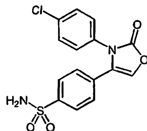
4-[3-(4-chlorophenyl)-2,3-dihydro-2-oxo-4-oxazolyl]benzenesulfonamide; C24)
