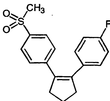
1-fluoro-4-[2-[4-(methylsulfonyl)phenyl]cyclopenten-1-yl]benzene; C19)
