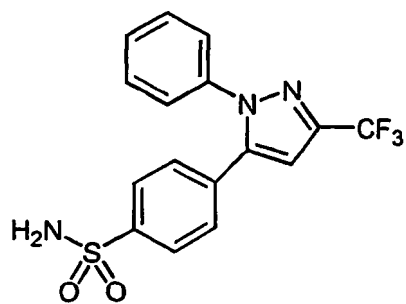
4-[1-phenyl-3-(trifluoromethyl)-1H-pyrazol-5-yl]benzenesulfonamide; C17)
