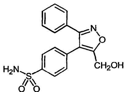
4-[5-(hydroxymethyl)-3-phenylisoxazol-4-yl]benzenesulfonamide; C23)
