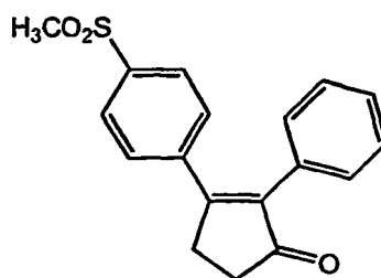
3-[4-(methylsulfonyl)phenyl]-2-phenyl-2-cyclopenten-1-one; C12)
