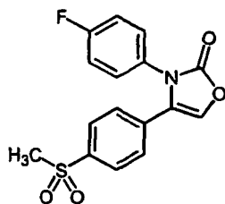
3-(4-fluorophenyl)-4-[4-(methylsulfonyl)phenyl]-2(3H)-oxazolone; C14)
