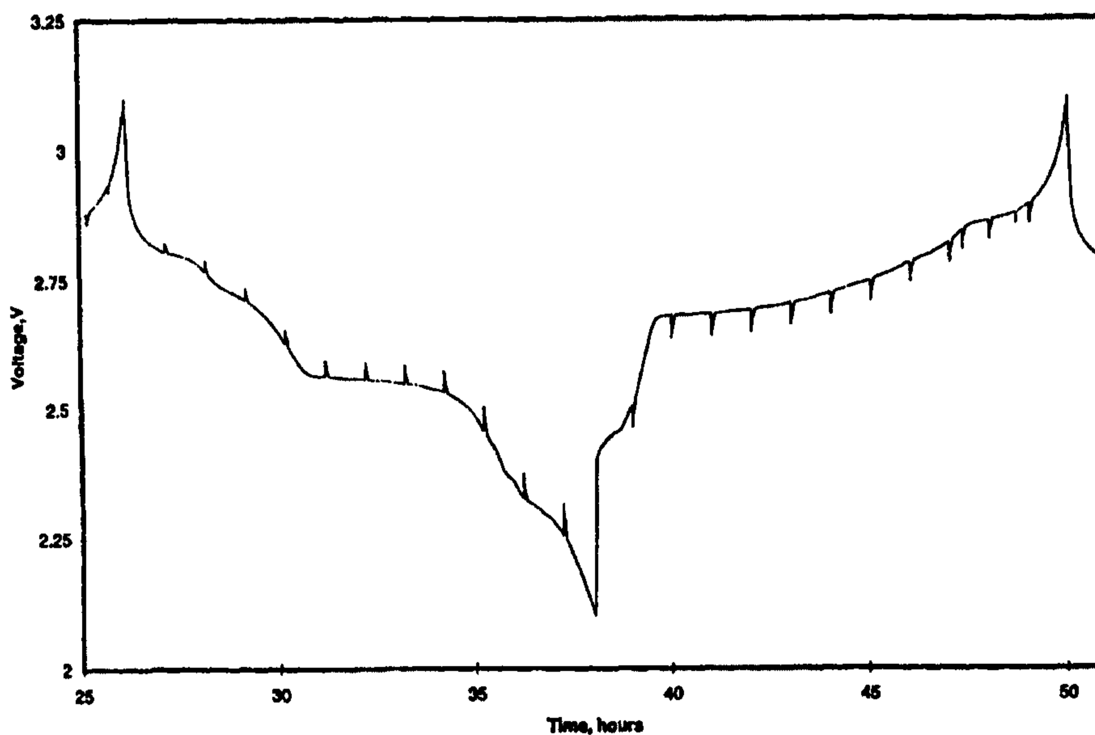
Voltage Curve \text{Li}_{1.2}\text{V}_3\text{O}_8
